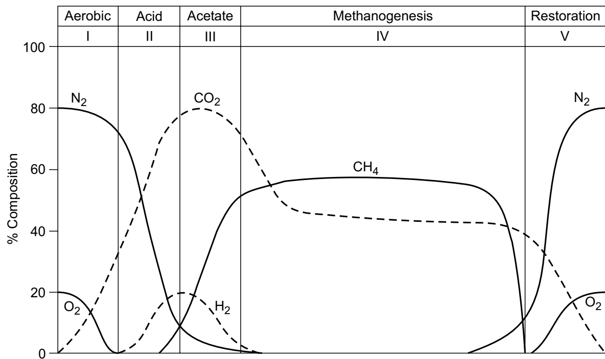
Figure 6 Typical changes in landfill gas composition with respect to the five phases of the landfill life-cycle (from Swarbrick, 2001).
