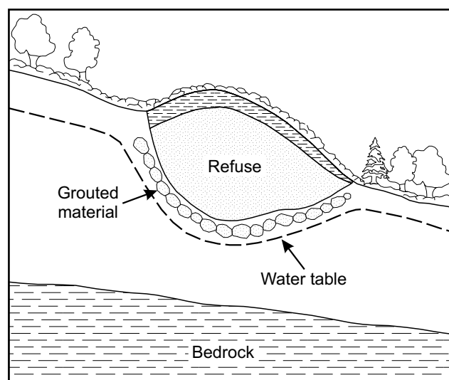
Figure 8 Application of grouting in the remediation of landfills (from Fetter, 1994).
