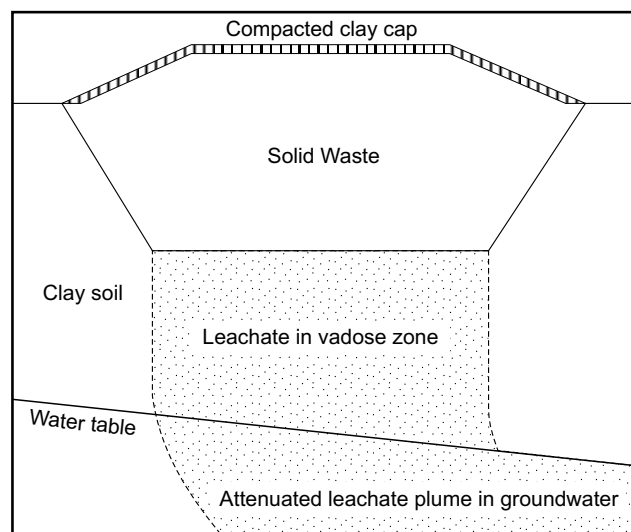
Figure 7 Natural attenuation of landfill leachate (from Fetter, 1994).
