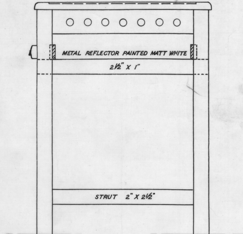
SIDE ELEVATION
