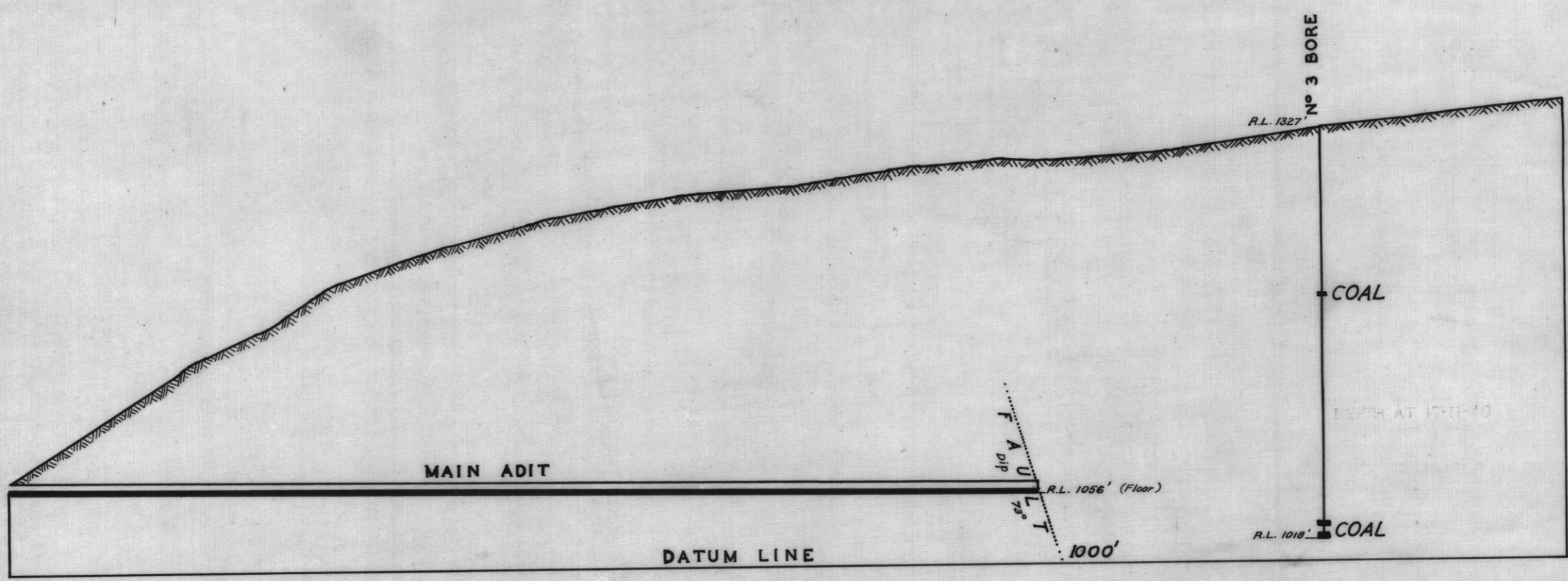
SECTION ALONG LINE OF MAIN ADIT TO N°3 BORE
