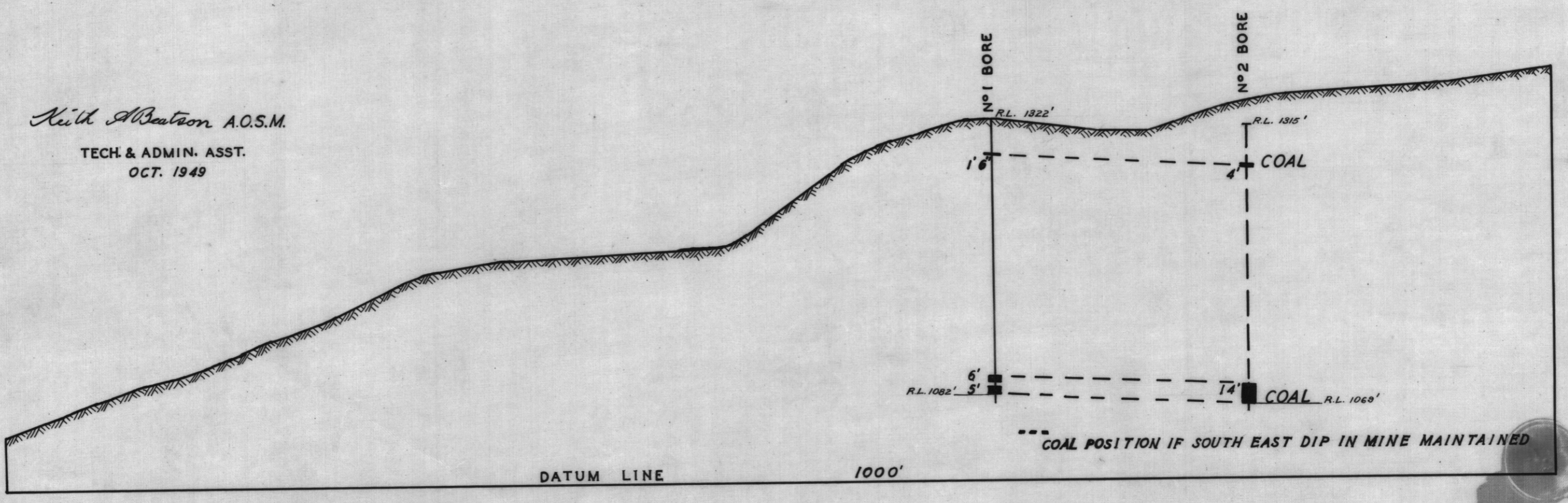
SECTION PARALLEL TO MAIN ADIT THROUGH N°1 BORE
