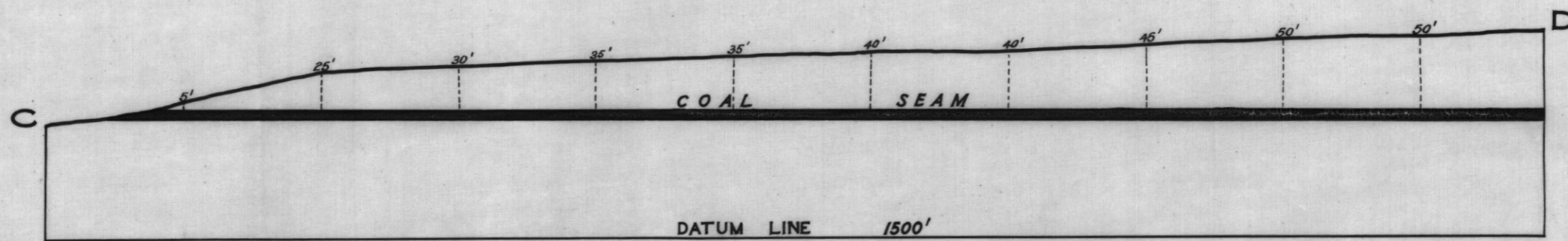
SECTION CD — ALONG STRIKE
