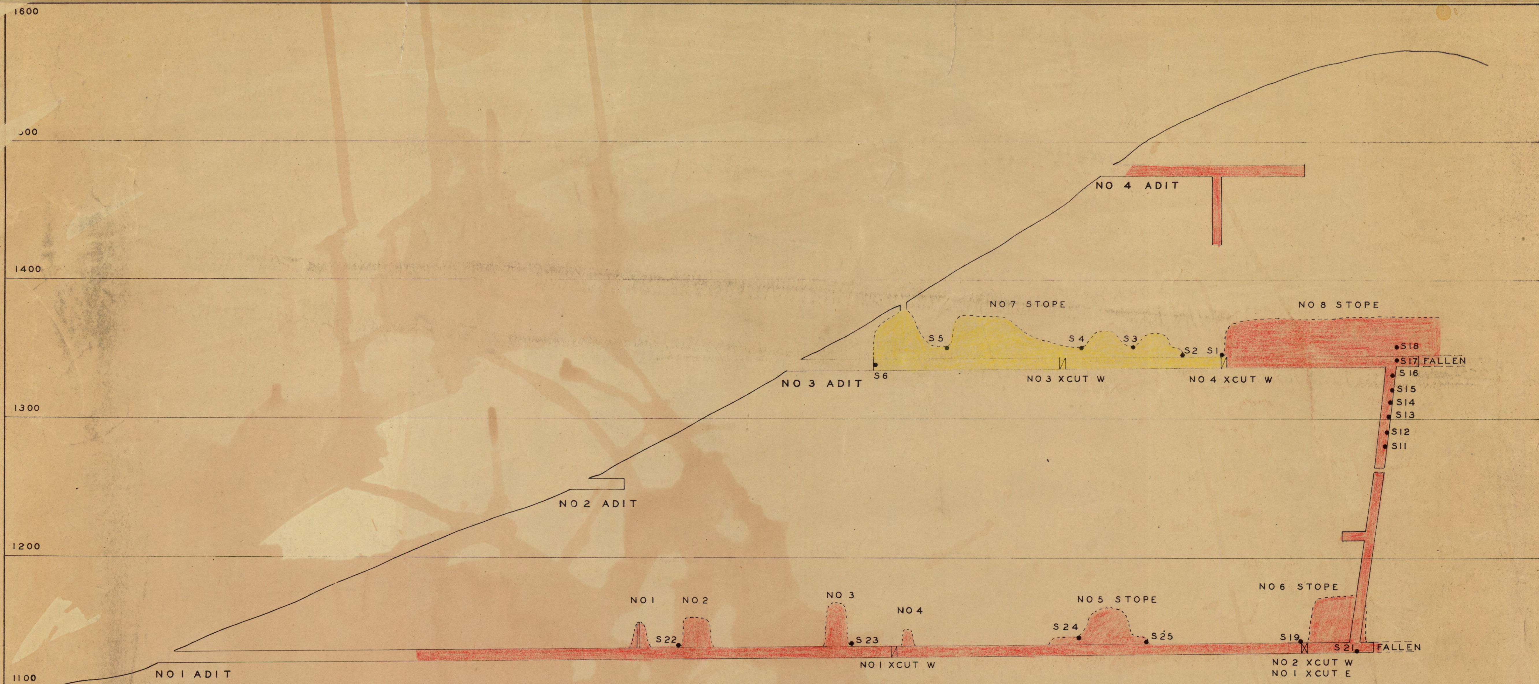
LONG SECTION PROJECTED ON TO AA' - LOOKING EAST
