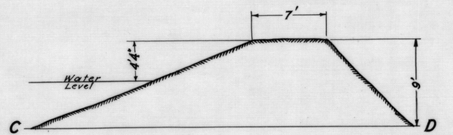
SECTION CD SCALE: 1 IN. = 10 FT.
