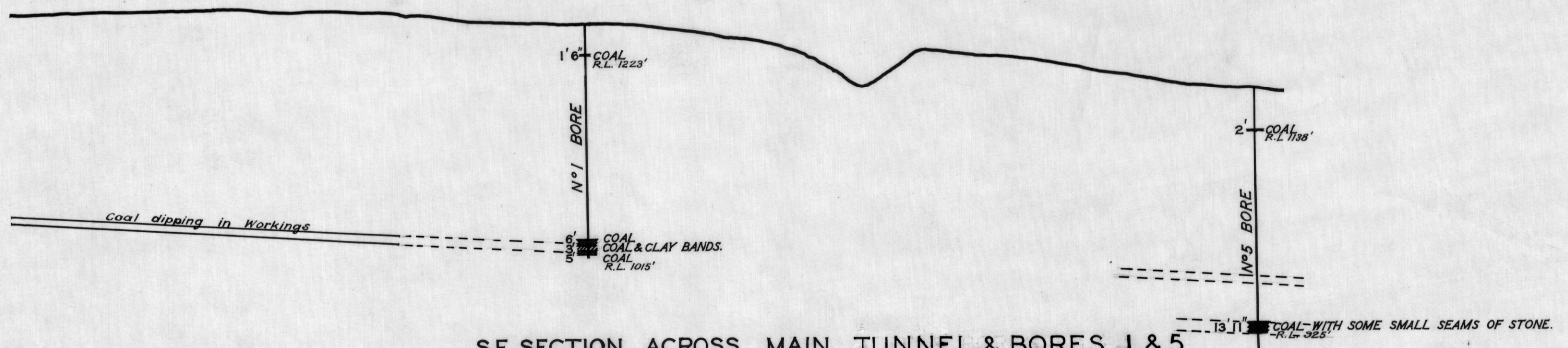
S.E. SECTION ACROSS MAIN TUNNEL & BORES 1 & 5 SECTION NO 3
