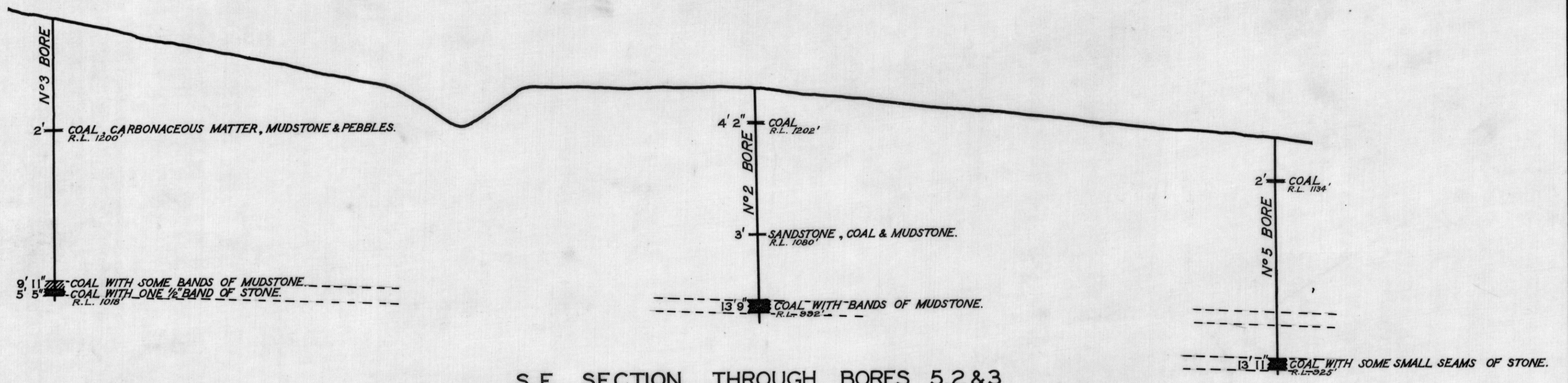
S.E. SECTION THROUGH BORES 5, 2 & 3 SECTION NO 1
