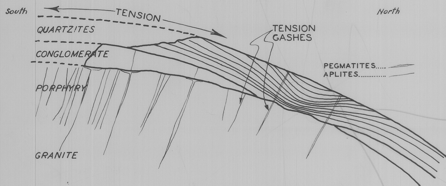
FIG. C (ii) AFTER GRANITE INTRUSION
