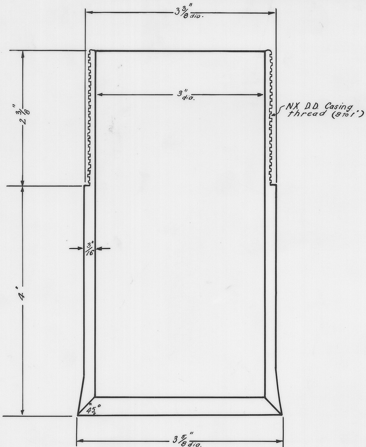
CUTTING SHOE
