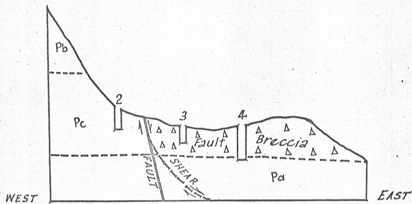
FIG. 2 SKETCH SECTION E-W N o 1 SITE
