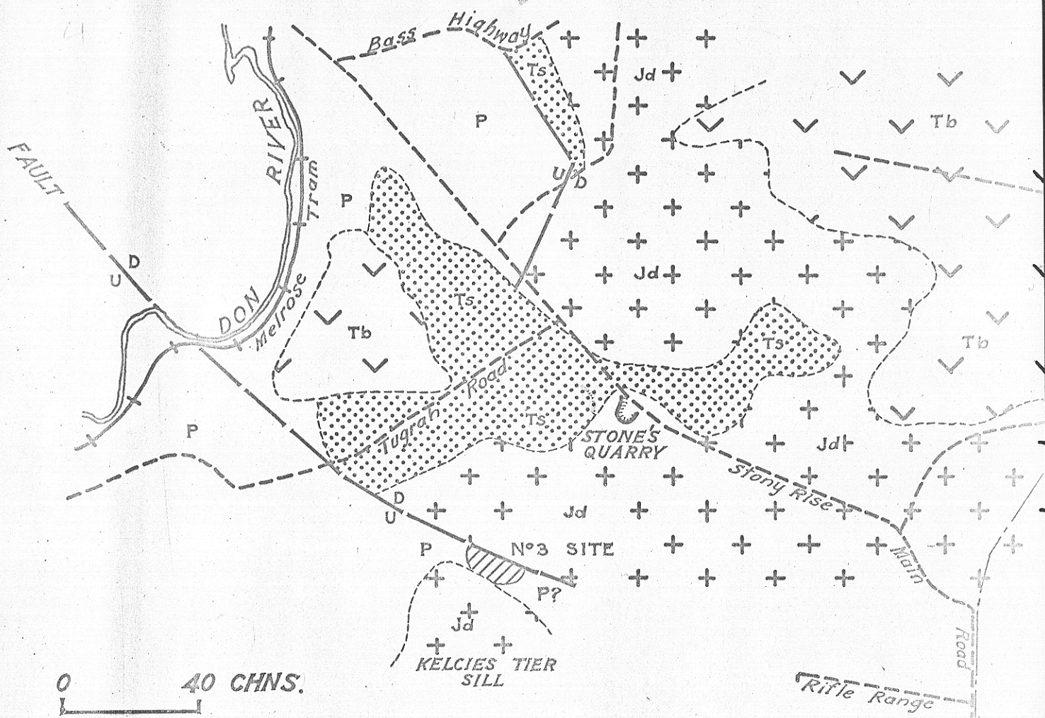
FIG. 9 PLAN OF STONY RISE AREA
