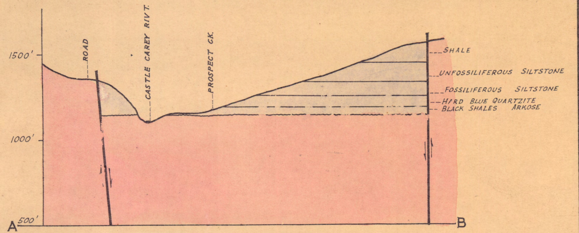
SECTION AB
