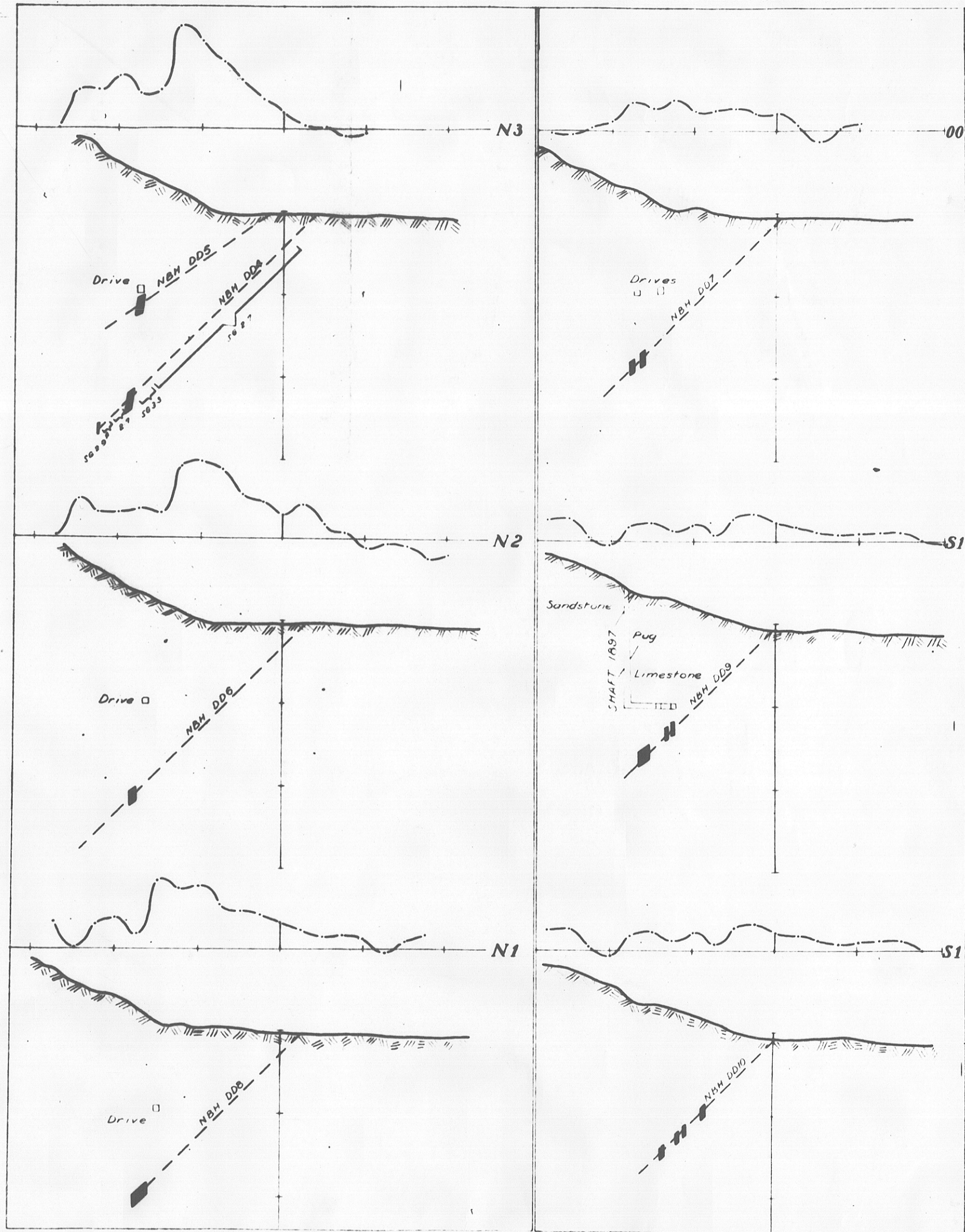
GEOPHYSICAL SURVEY AT ZEEHAN TASMANIA MARIPOSA AREA VERTICAL SECTIONS THROUGH DIAMOND DRILL HOLES SHOWING RELATIONS TO GRAVITY ANOMALIES.
