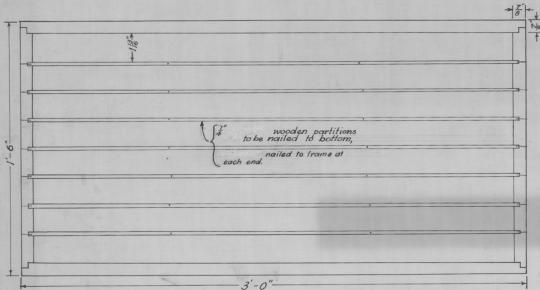
PLAN
