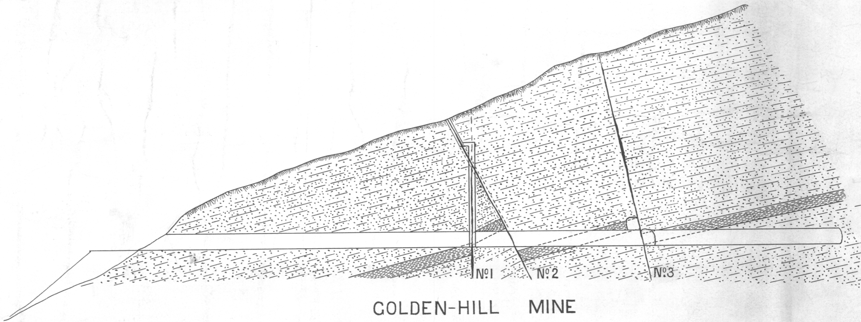
SECTIONAL SKETCH OF COUNTRY AND MINE-WORKINGS
