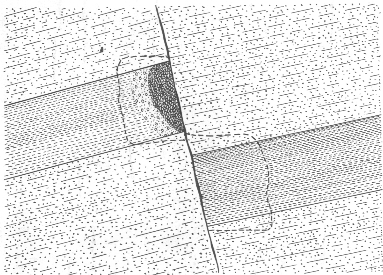
ENLARGED SECTION ON FORMATION N o 3 NOT TO SCALE
