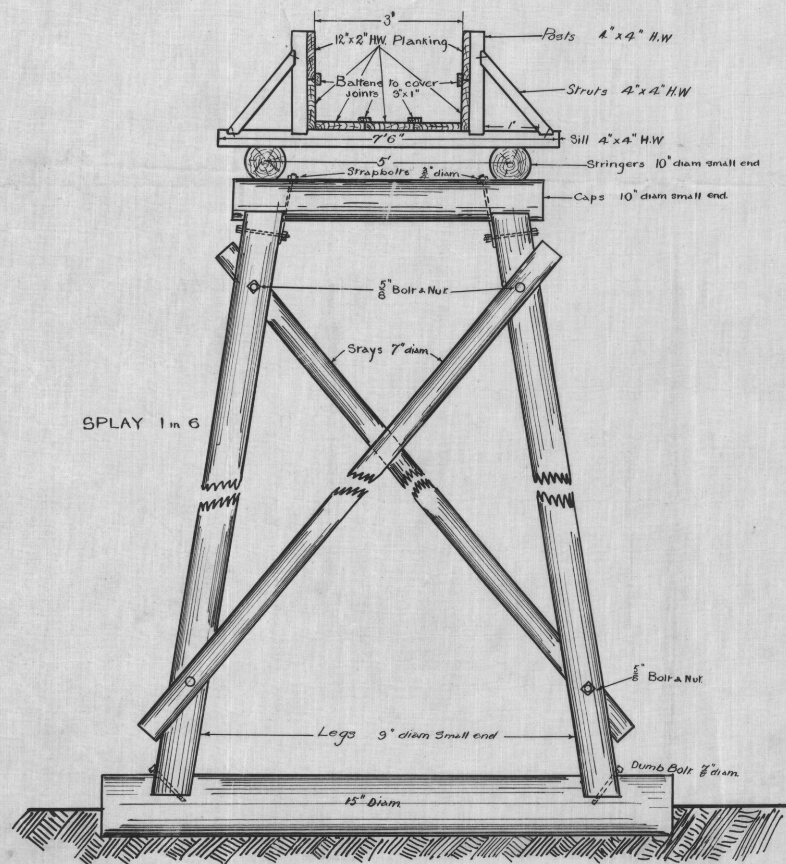
SECTION OF FLUME AND TRESTLE
