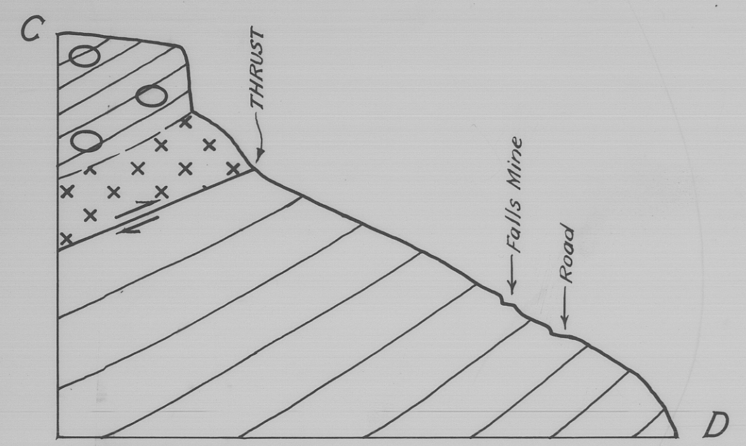
SECTION CD N.B. BEDDING INTERPRATIVE ONLY
