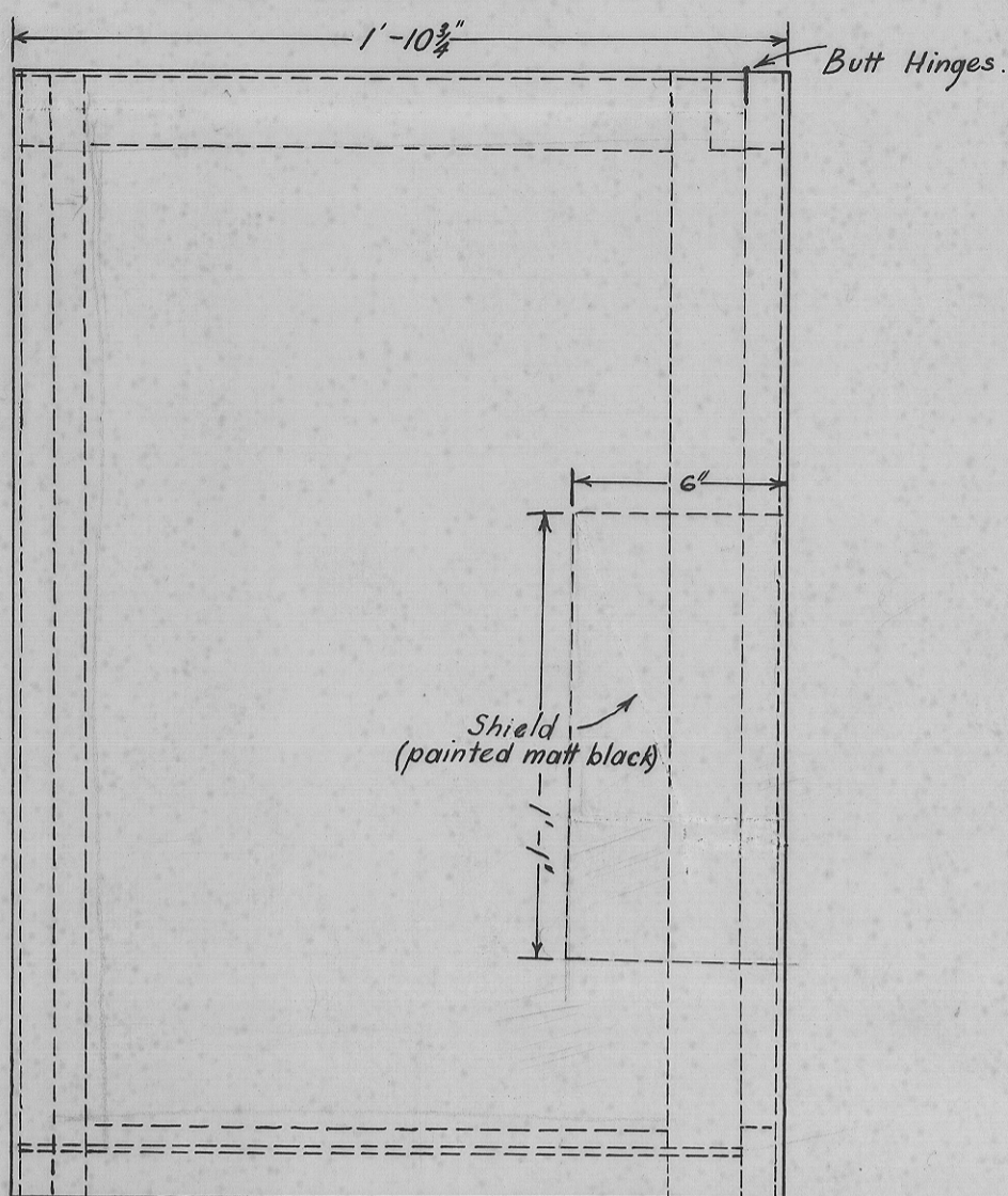
CABINET SIDE ELEVATION
