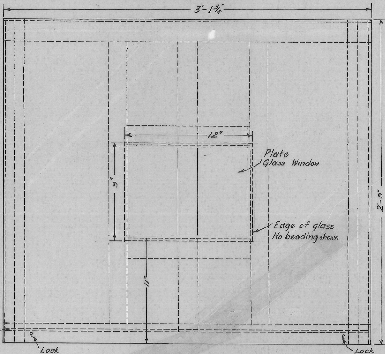
CABINET ELEVATION
