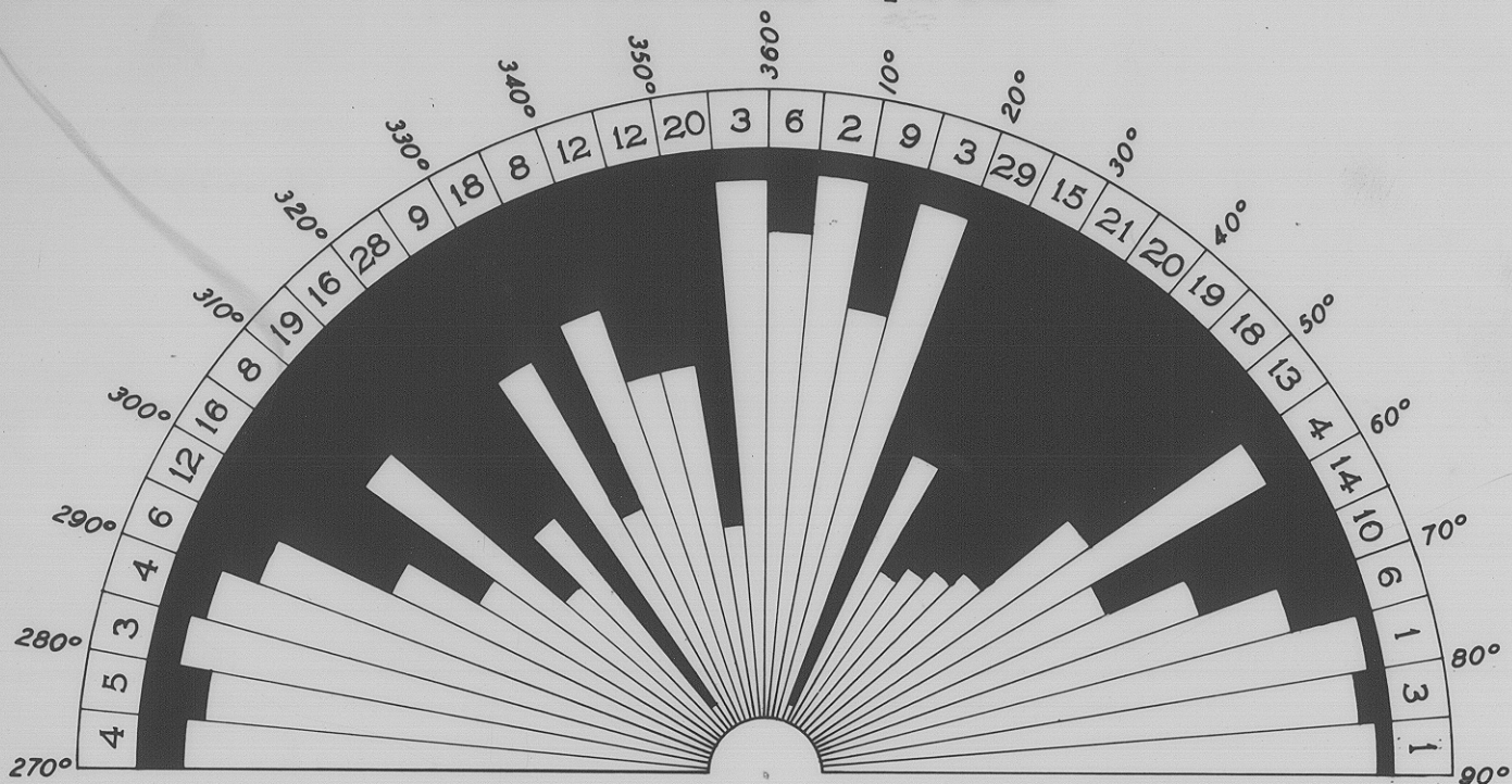
JOINTS 0°-90° GOLIATH CEMENT COY'S QUARRY
