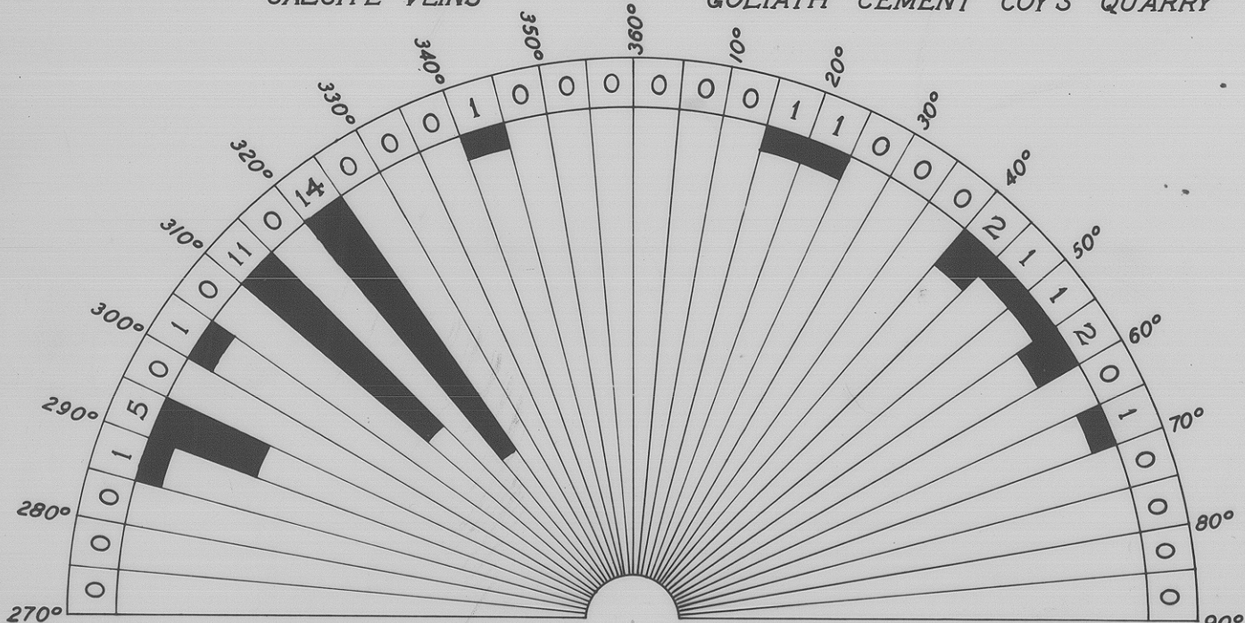
JOINTS 0°-90° BLENKHORNS QUARRY
