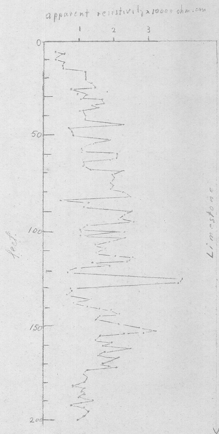
Three electrode Resistivity log Drill hole at bottom of quarry.
