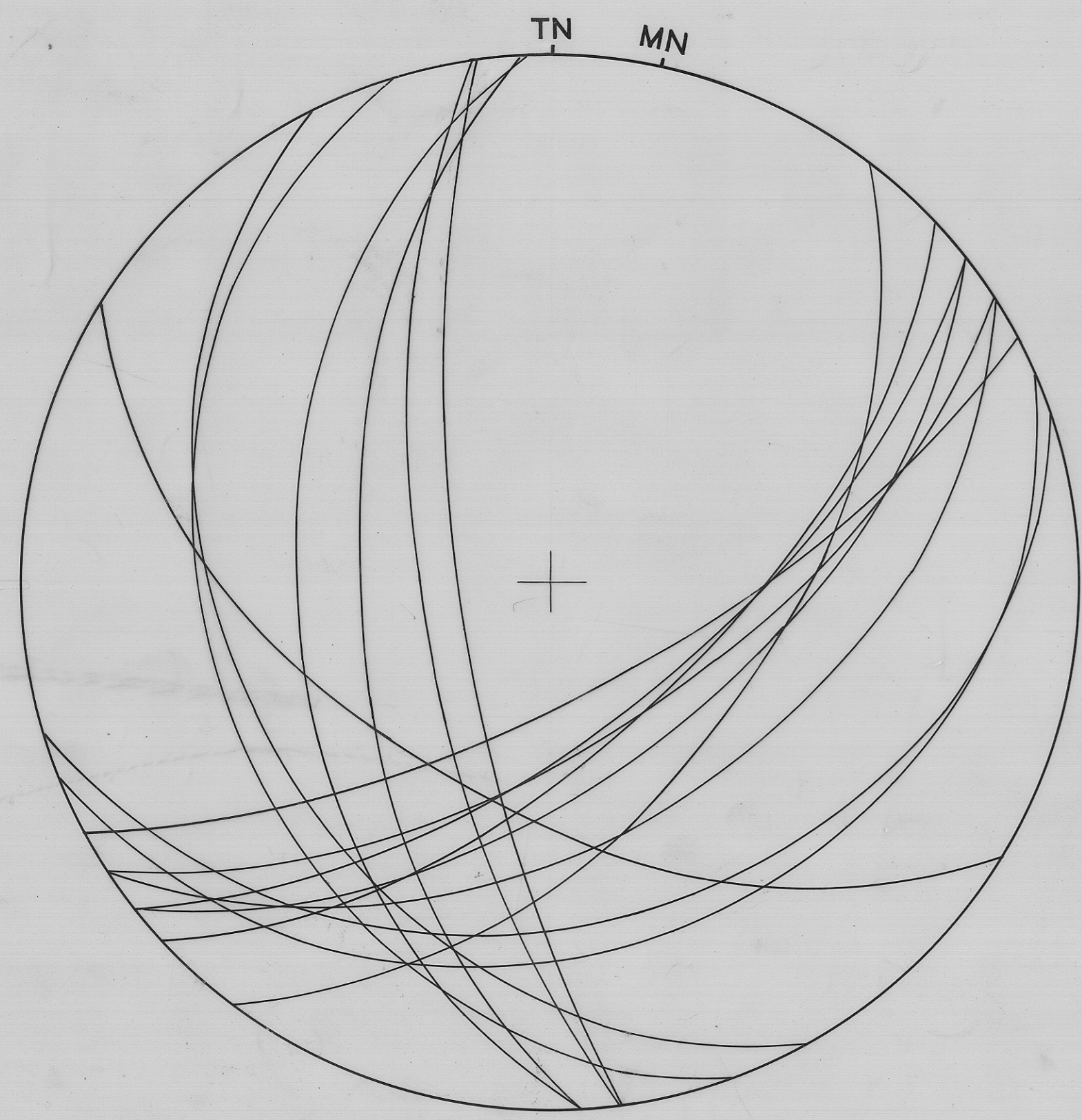
BEDDING - ELLIS TUNNEL
