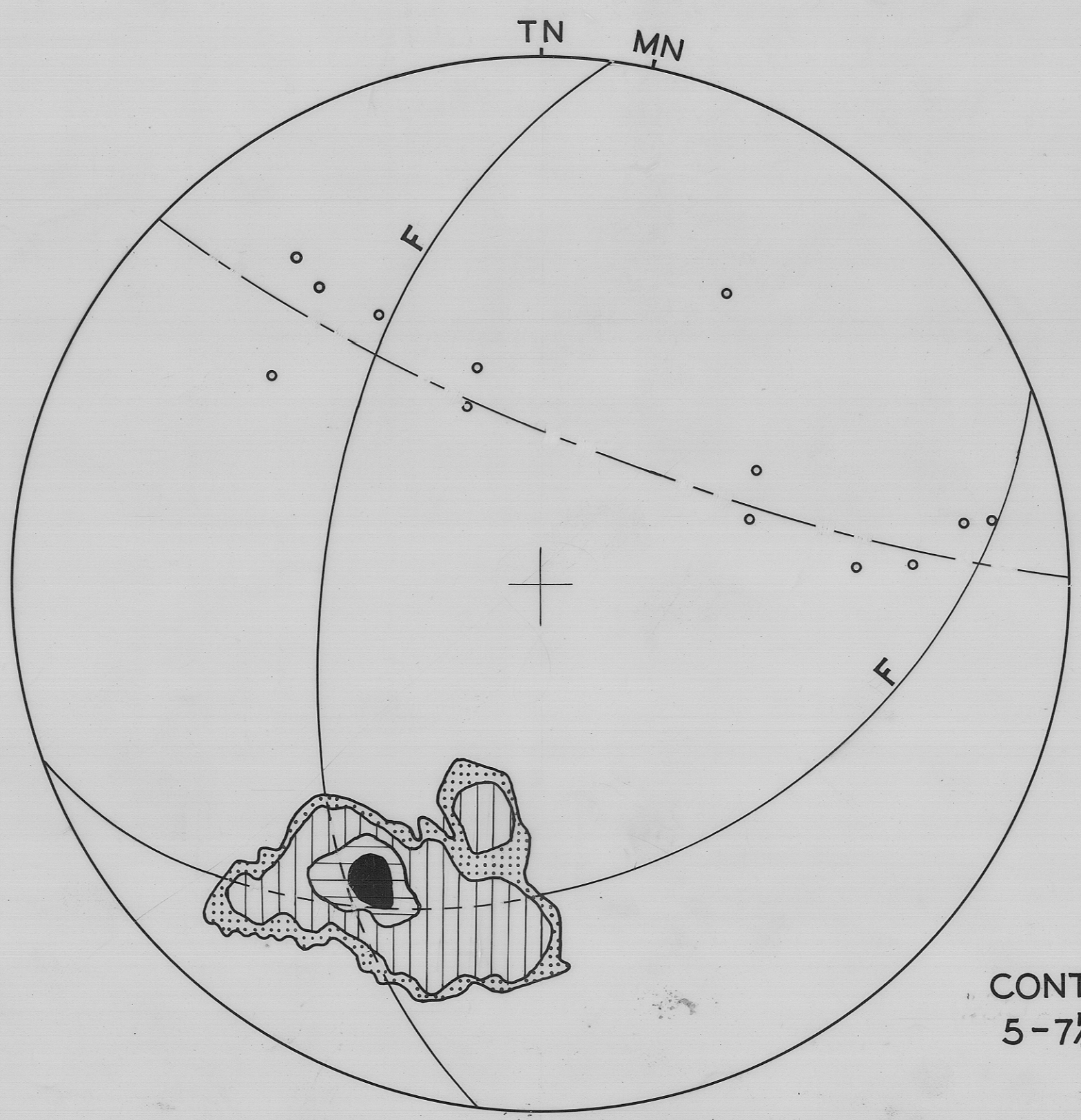
IRON CLIFFS ANTICLINE - BEDDING INTERSECTIONS
