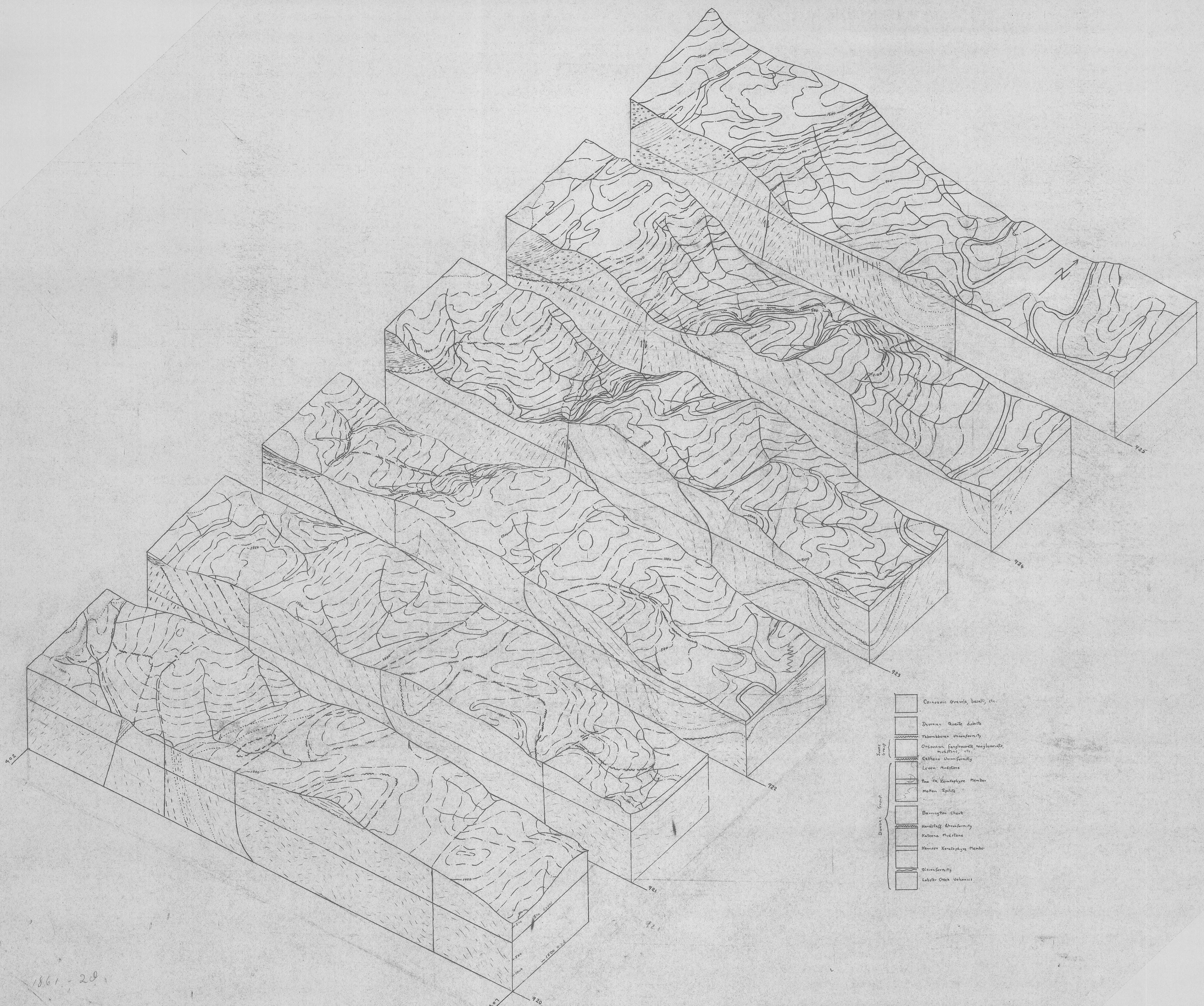
STEREOGRAM OF MT. YOUNG
