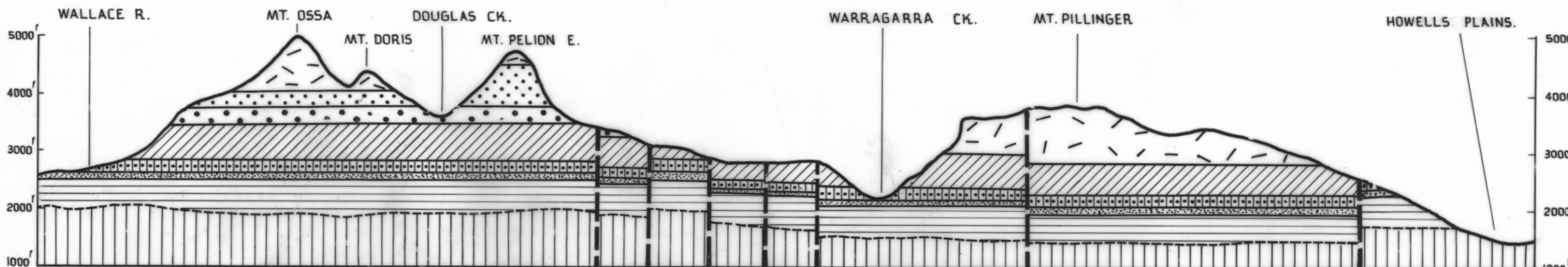
SECTION ON LINE C-D WALLACE RIVER TO HOWELLS PLAINS
