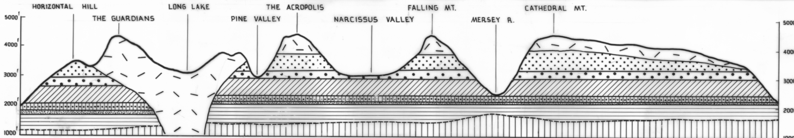
SECTION ON LINE A-B HORIZONTAL HILL TO CATHEDRAL MOUNTAIN
