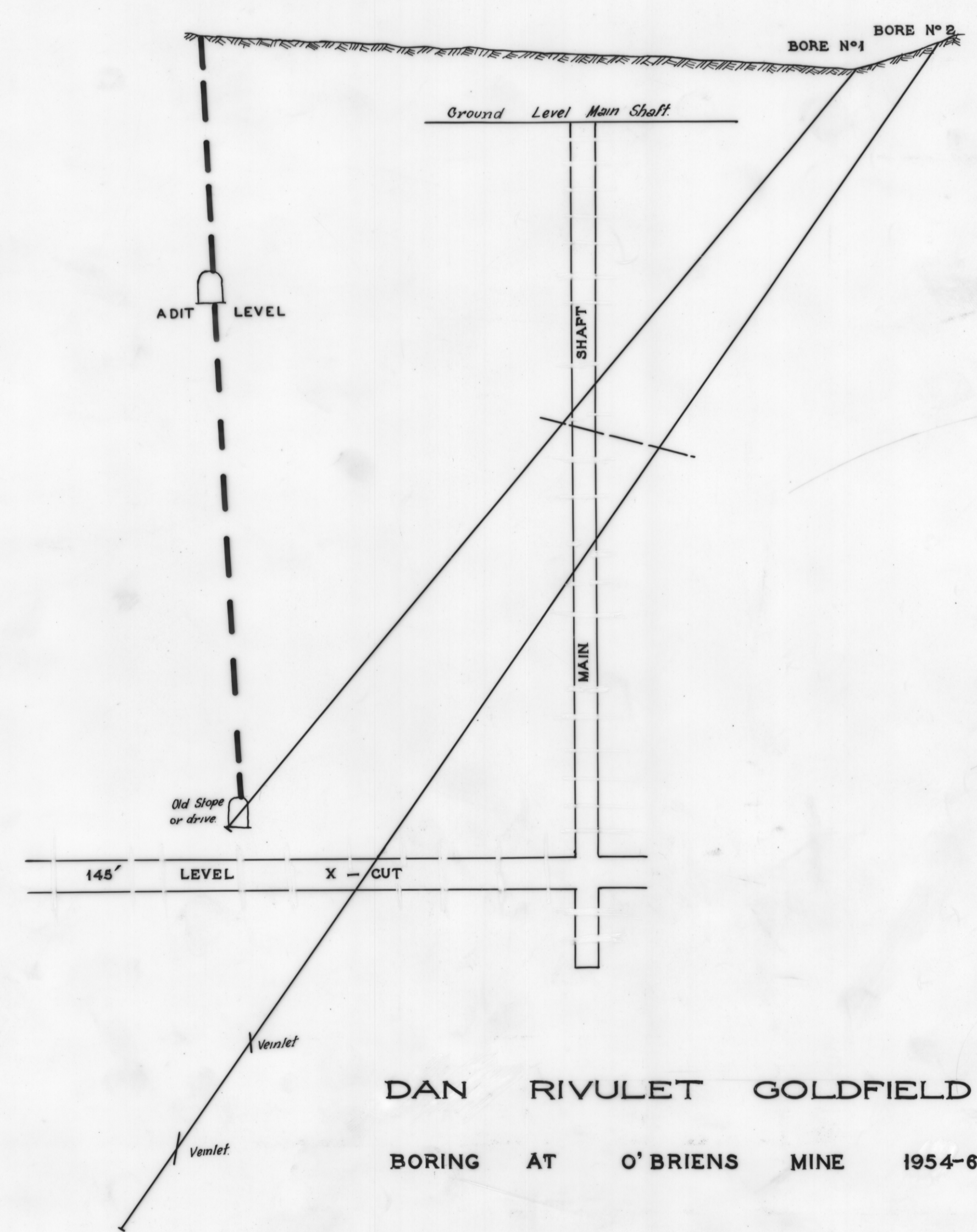
SECTION ALONG BORE N° 1 LOOKING N.E.
