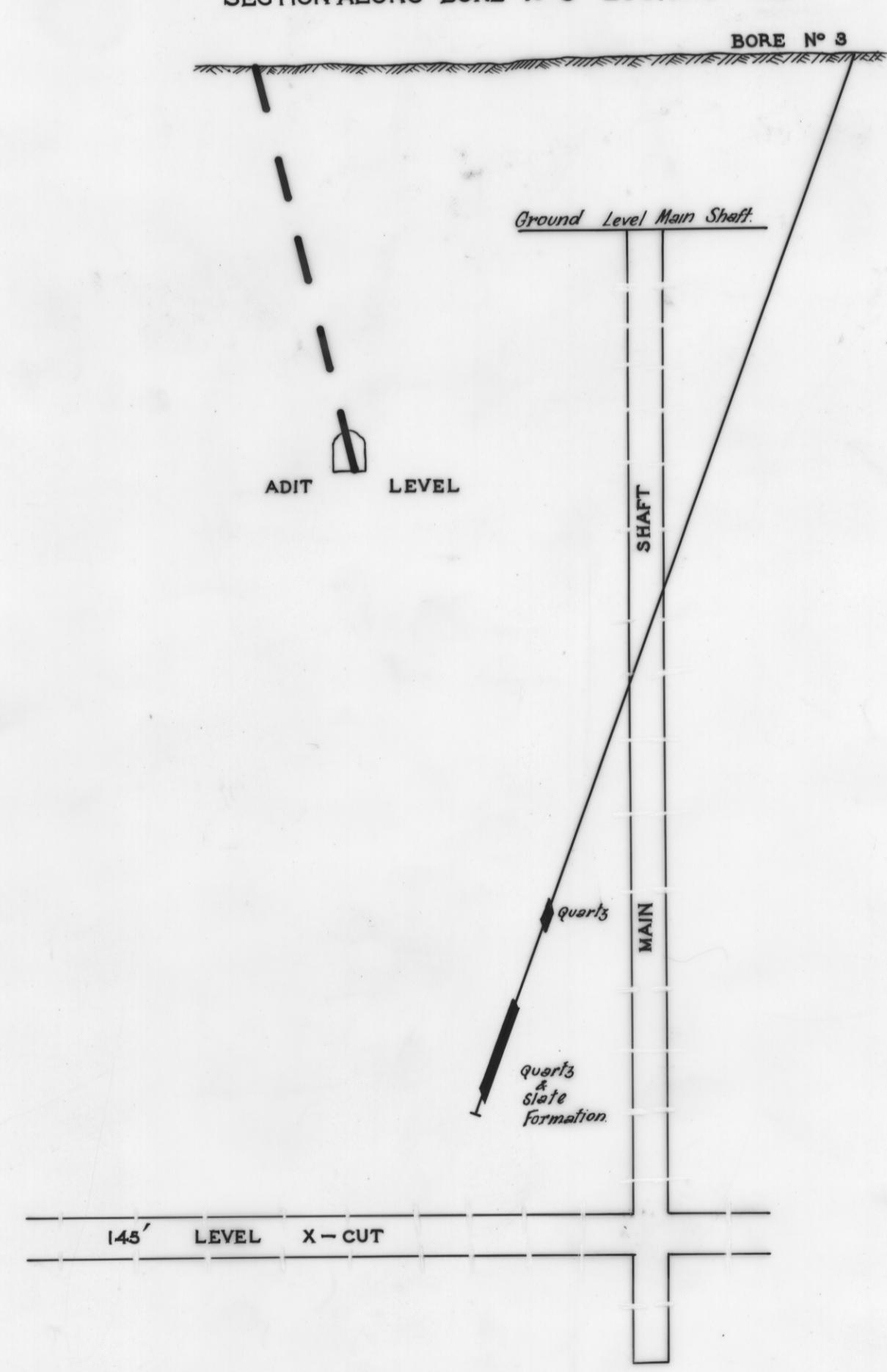
SECTION ALONG BORE N° 3 LOOKING N.E.
