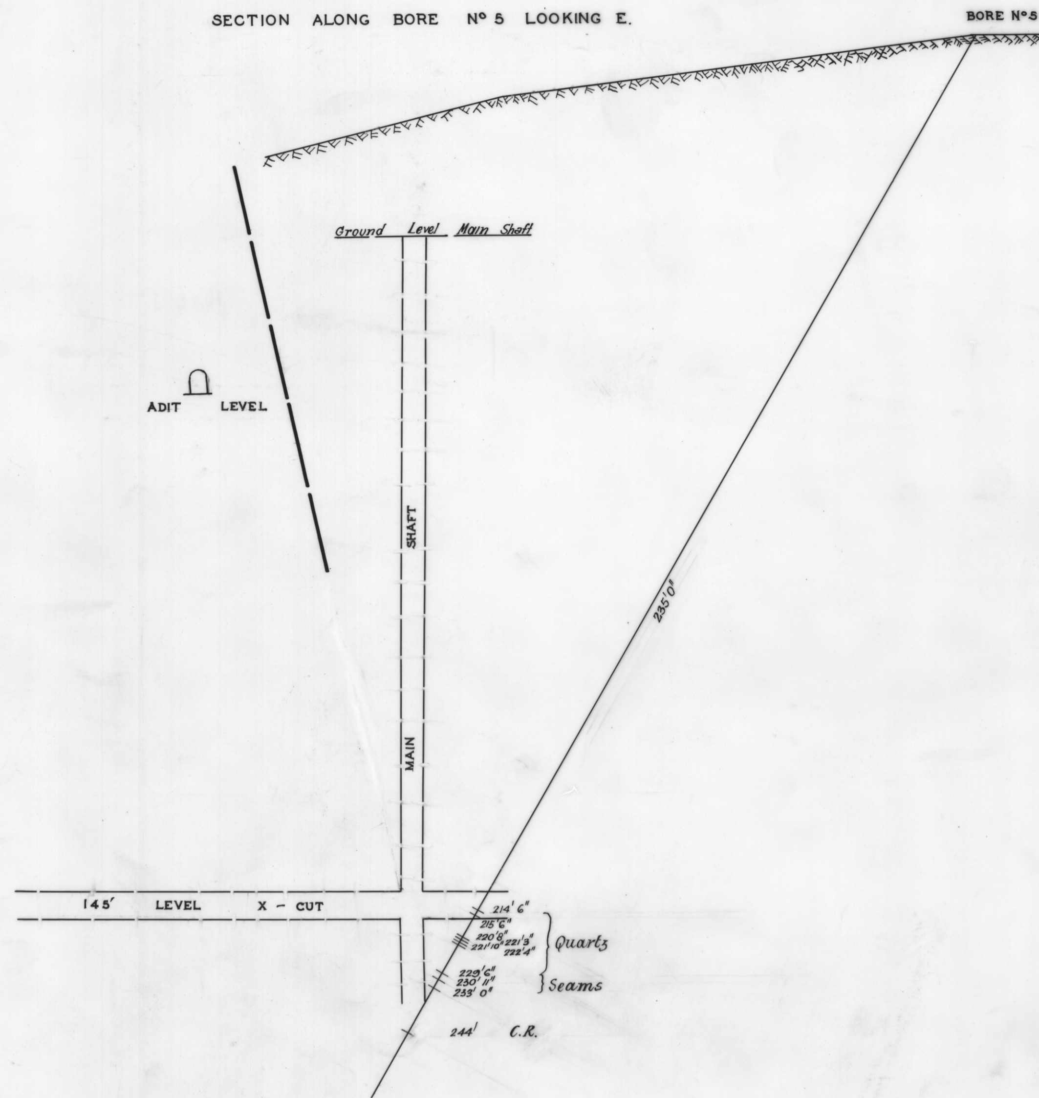
SECTION ALONG BORE N° 5 LOOKING E.
