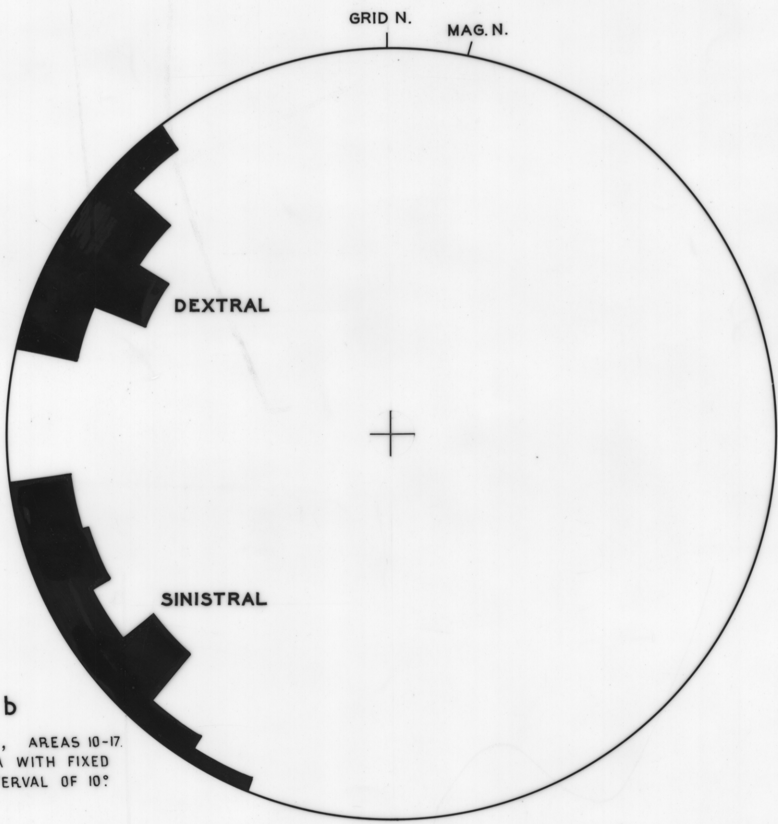
KNICK PLANES IN CONGLOMERATE
