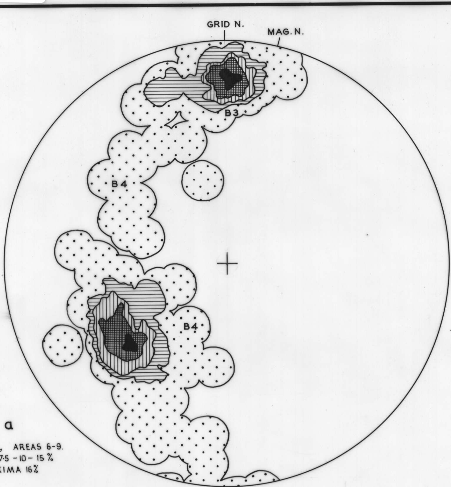
FLEXURAL FOLDS IN SCHIST
