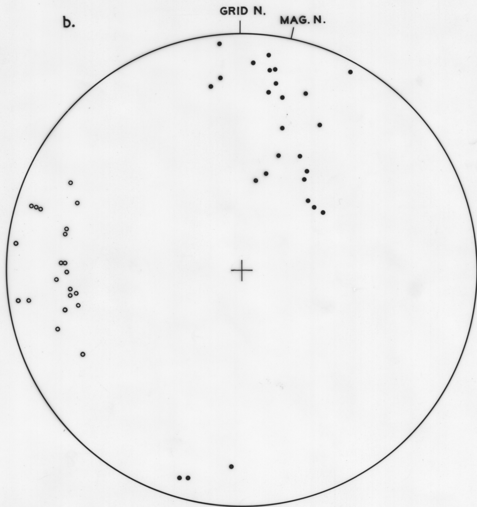
VERTICAL SHEARS • LINEATIONS ON SHEAR PLANES. • POLES OF SHEAR PLANES
