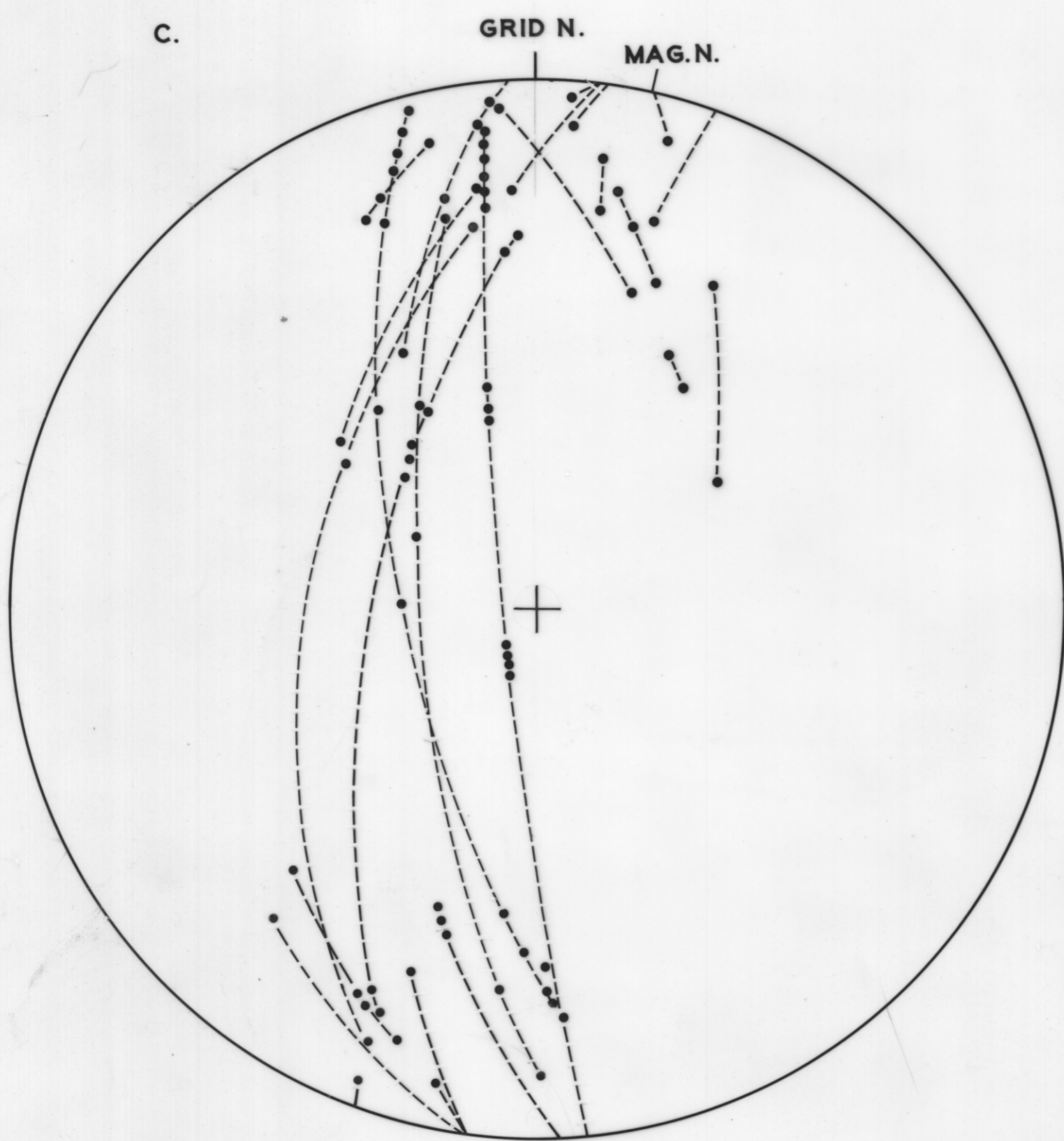
MULTIPLY LINEATED SURFACES —•— TRACES OF SHEAR PLANES WITH AXES OF LINEATION.
