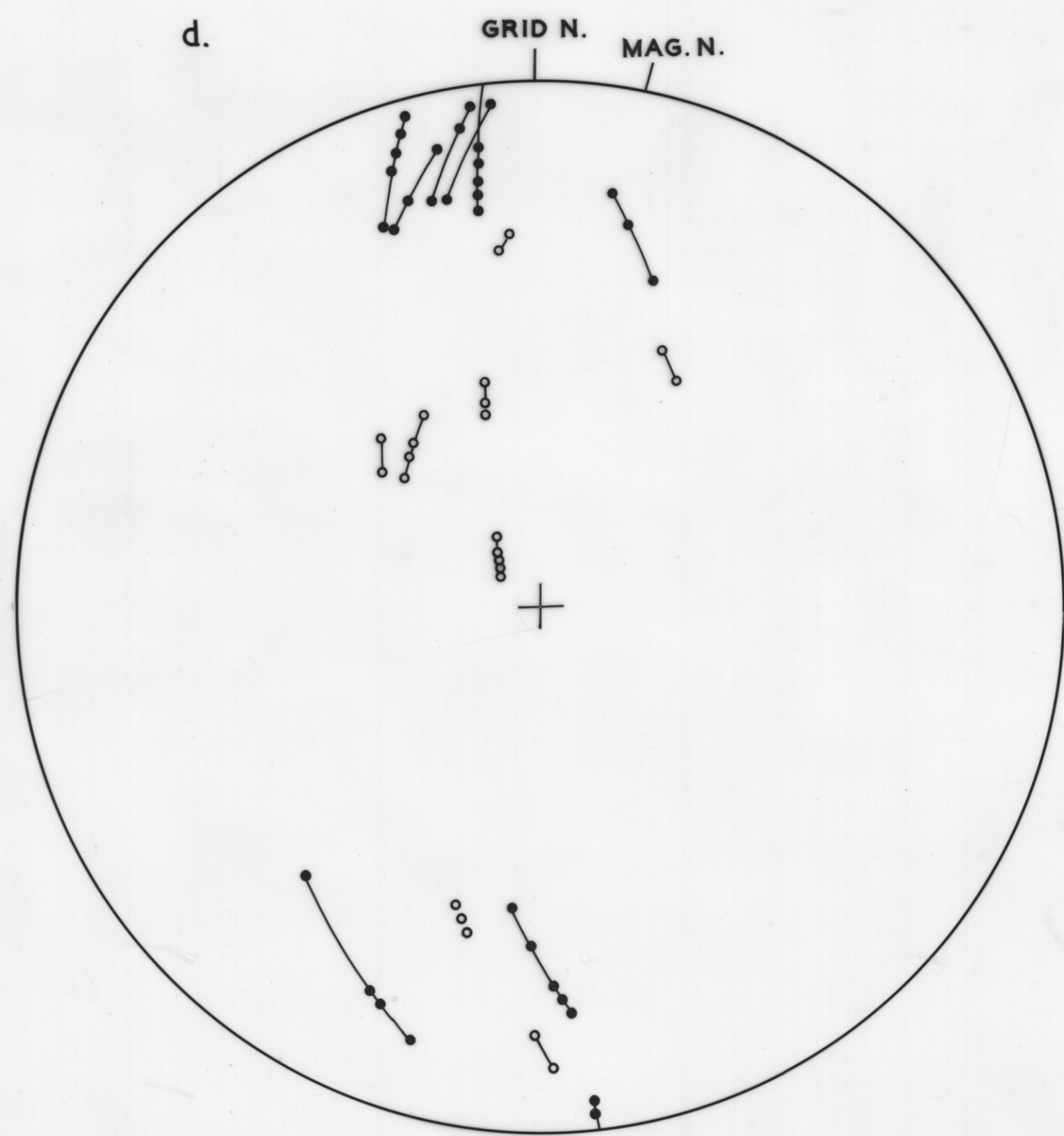
SETS OF LINEATIONS —•— TRACE OF SHEAR PLANE WITH AXES OF LINEATIONS. —○— RANGE OF SCATTERED NON-FOLDED LINEATIONS. —•— SAMPLES ALONG FOLDED LINEATIONS.
