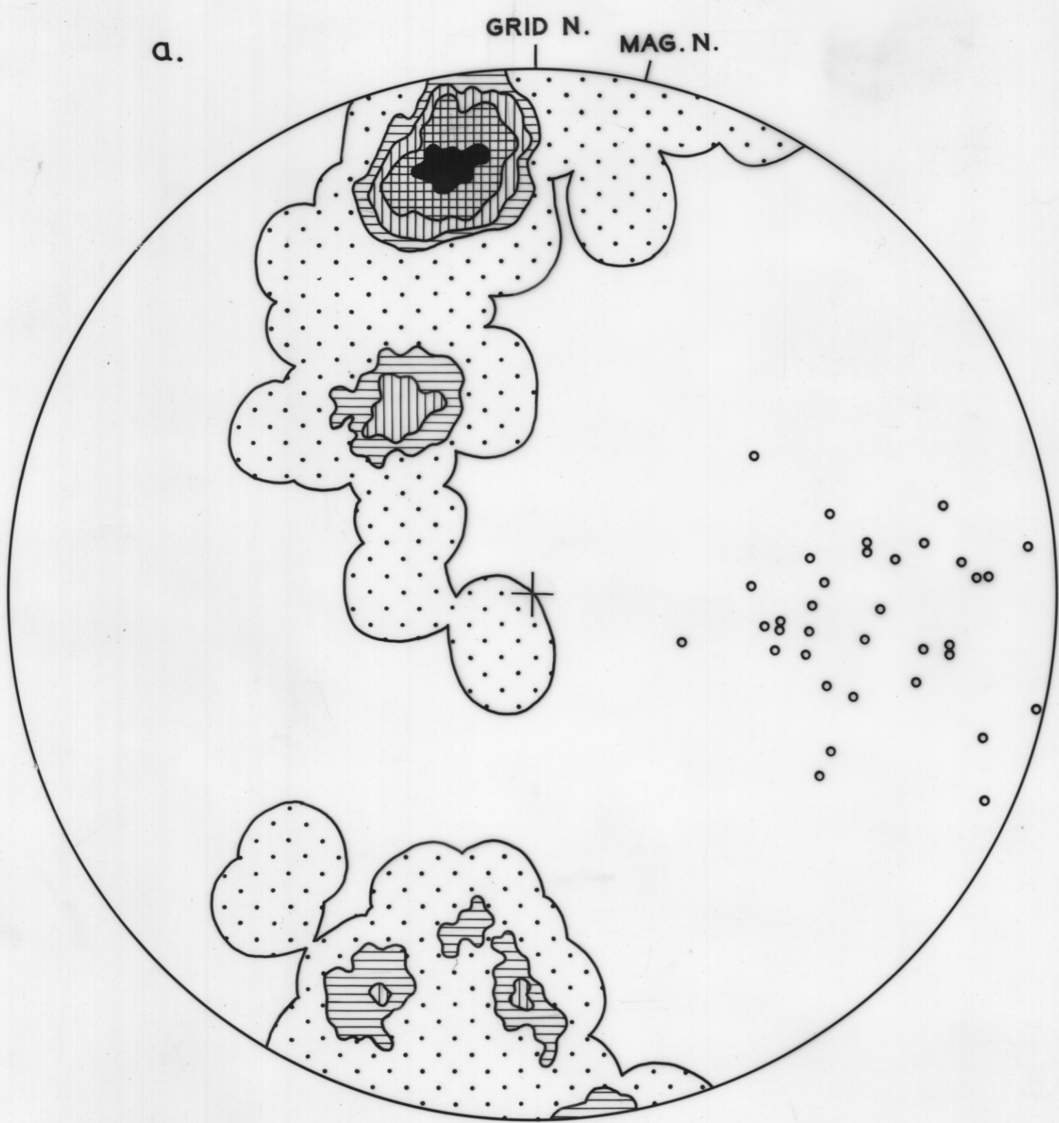
OBLIQUE SHEARS • POLES OF SHEAR PLANES CONTOURS OF 87 LINEATIONS. CONTOURS 0-5-7-10-15 % MAX. 17 %
