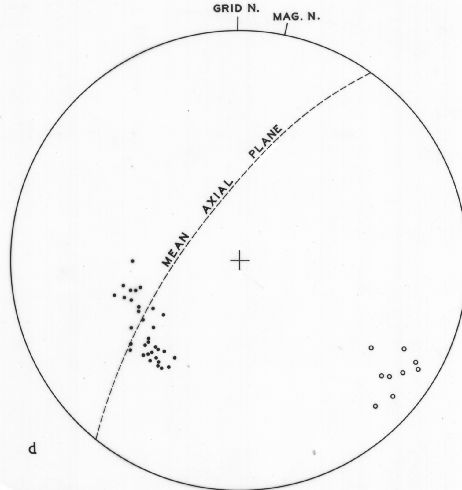
SUBAREAS 1, 2, 5. • POLES TO AXIAL PLANES • 33β (S 0 S 1 )
