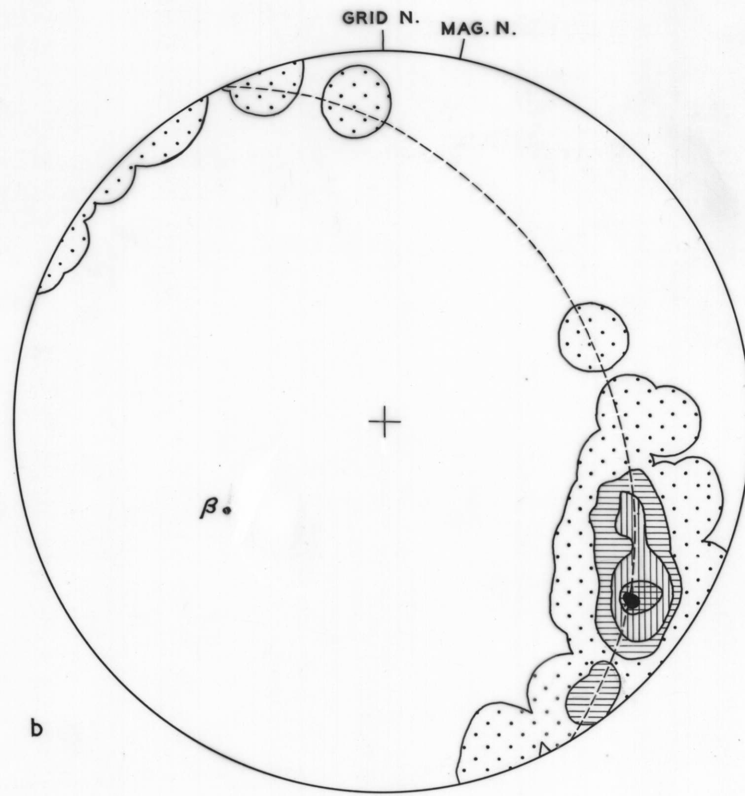
SUBAREA 2. 80 TS CONTOURS 0-10-20-25-27%
