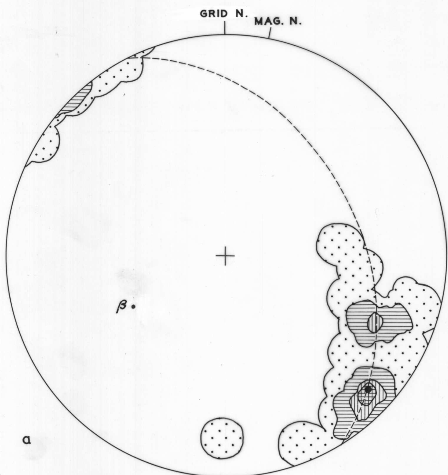
SUBAREA 1. 35 TS CONTOURS 0-10-20-25-29%
