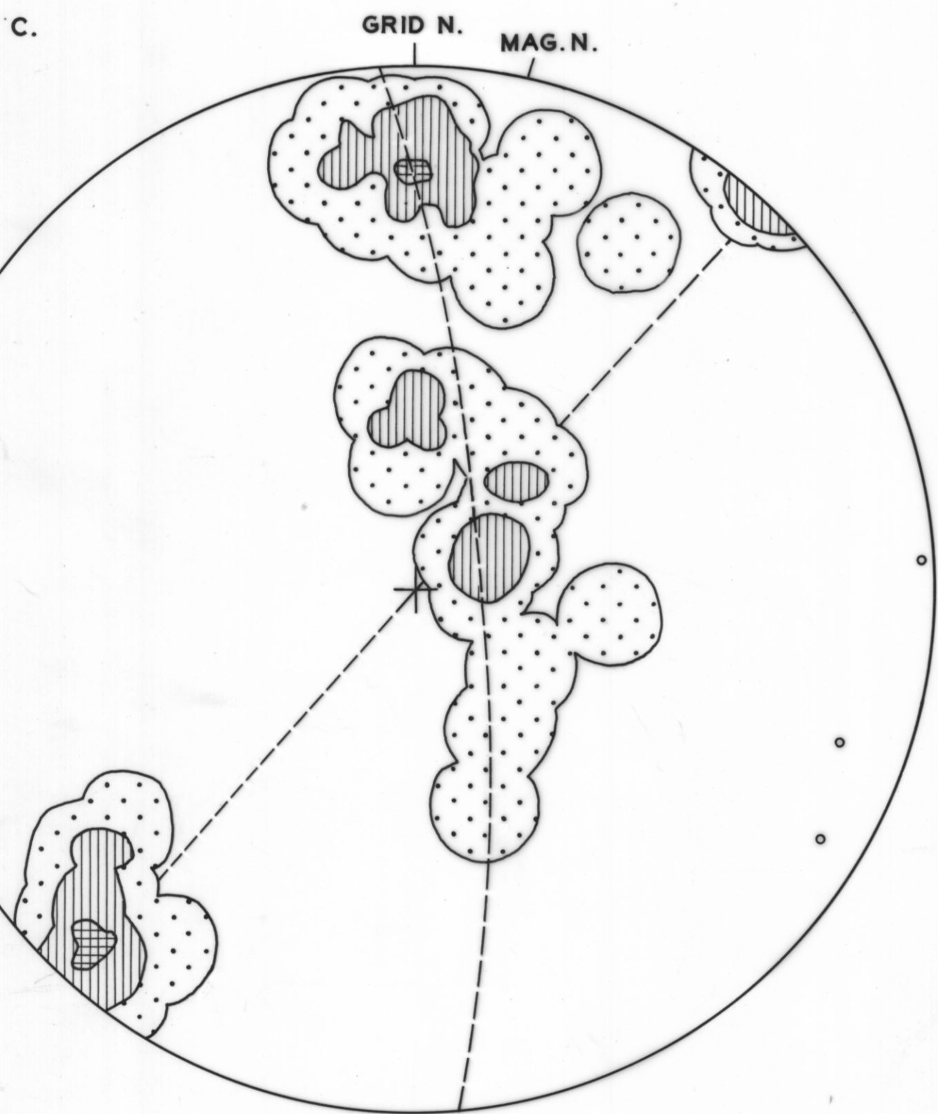
35 FOLD AXES CONTOURS 0-8-15 % ° AXIAL PLANES
