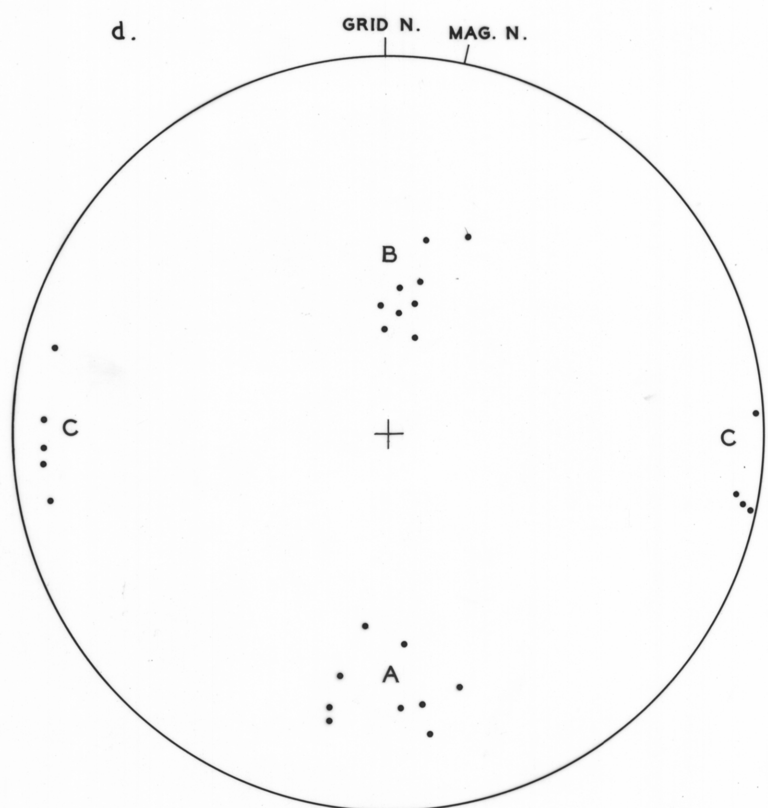
A,B,C, AXES OF SHEAR JOINTS 9 LOCALITIES
