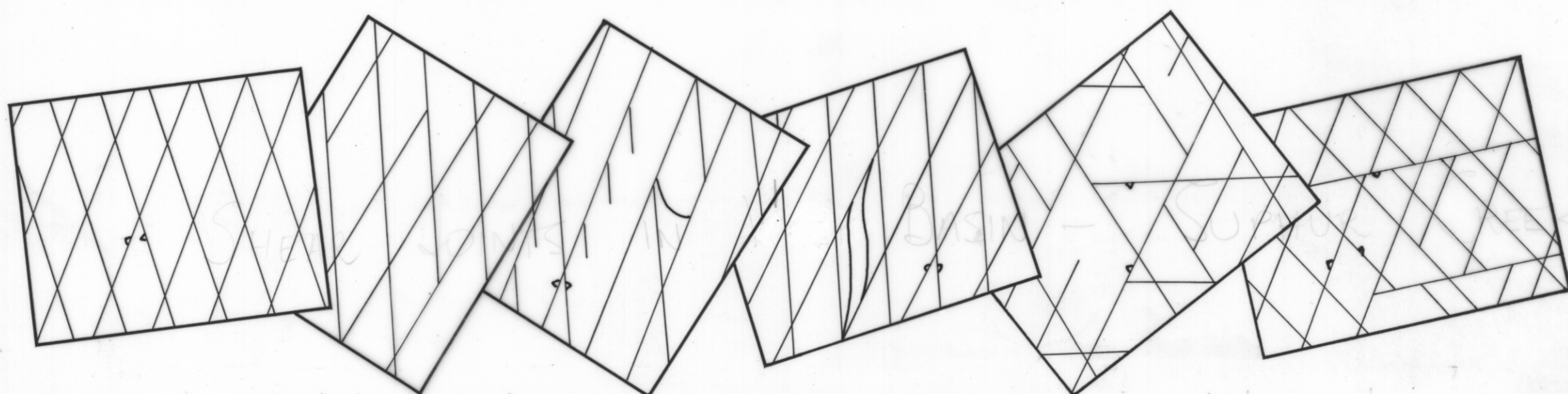
SHEAR JOINT PATTERN WEST LIMB OF EAST BASIN
