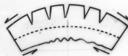
COMPETENT FOLDING
