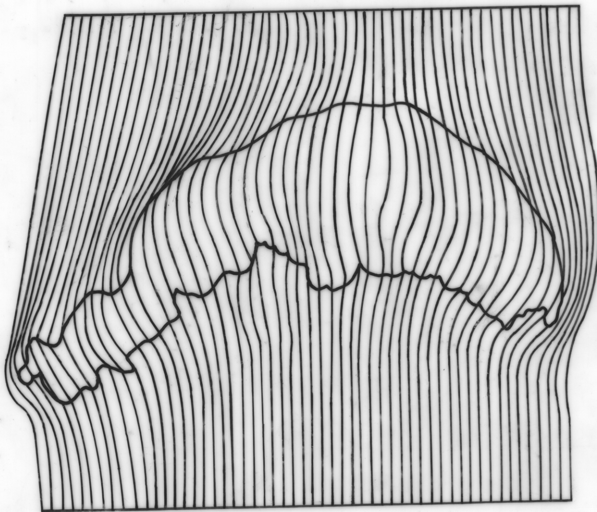
SECONDARY STRAINS
