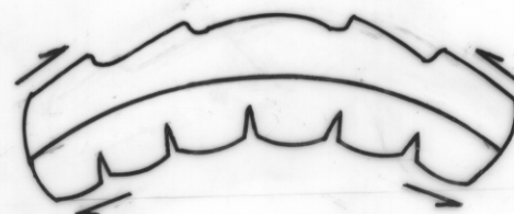
INCONGRUENT FOLDING
