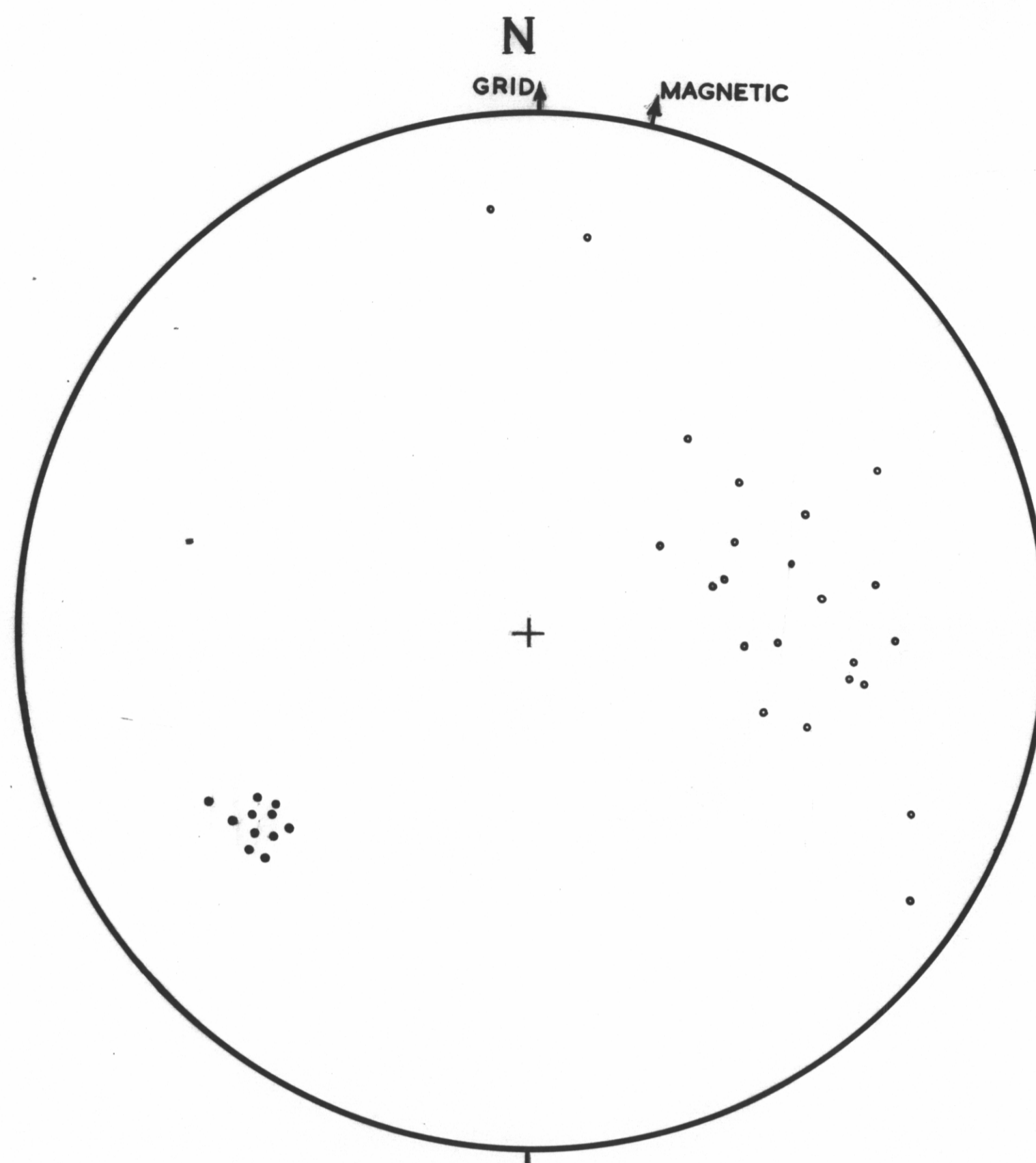
b. FRACTURE CLEAVAGE
