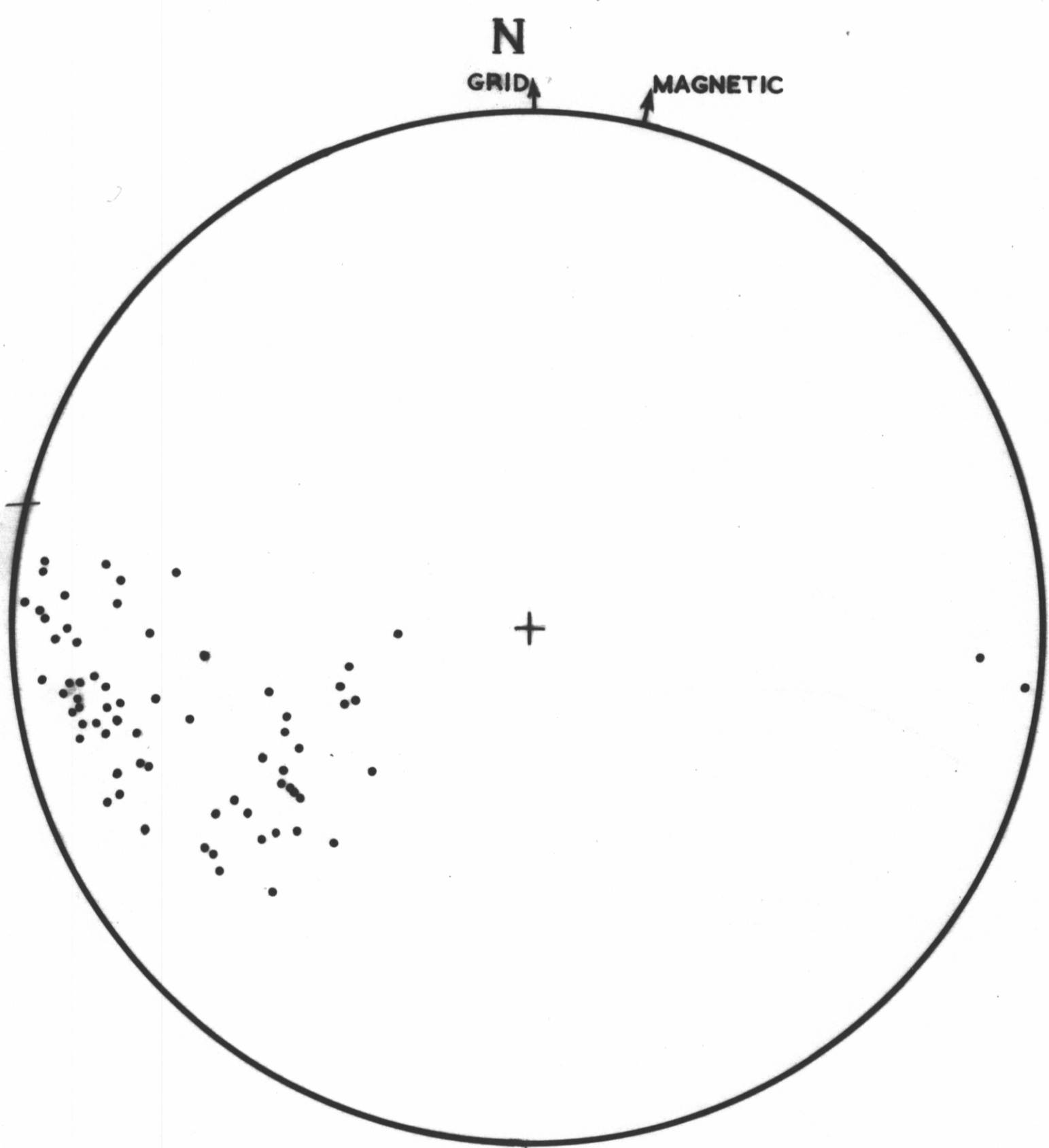
c. LINEATION L_1
