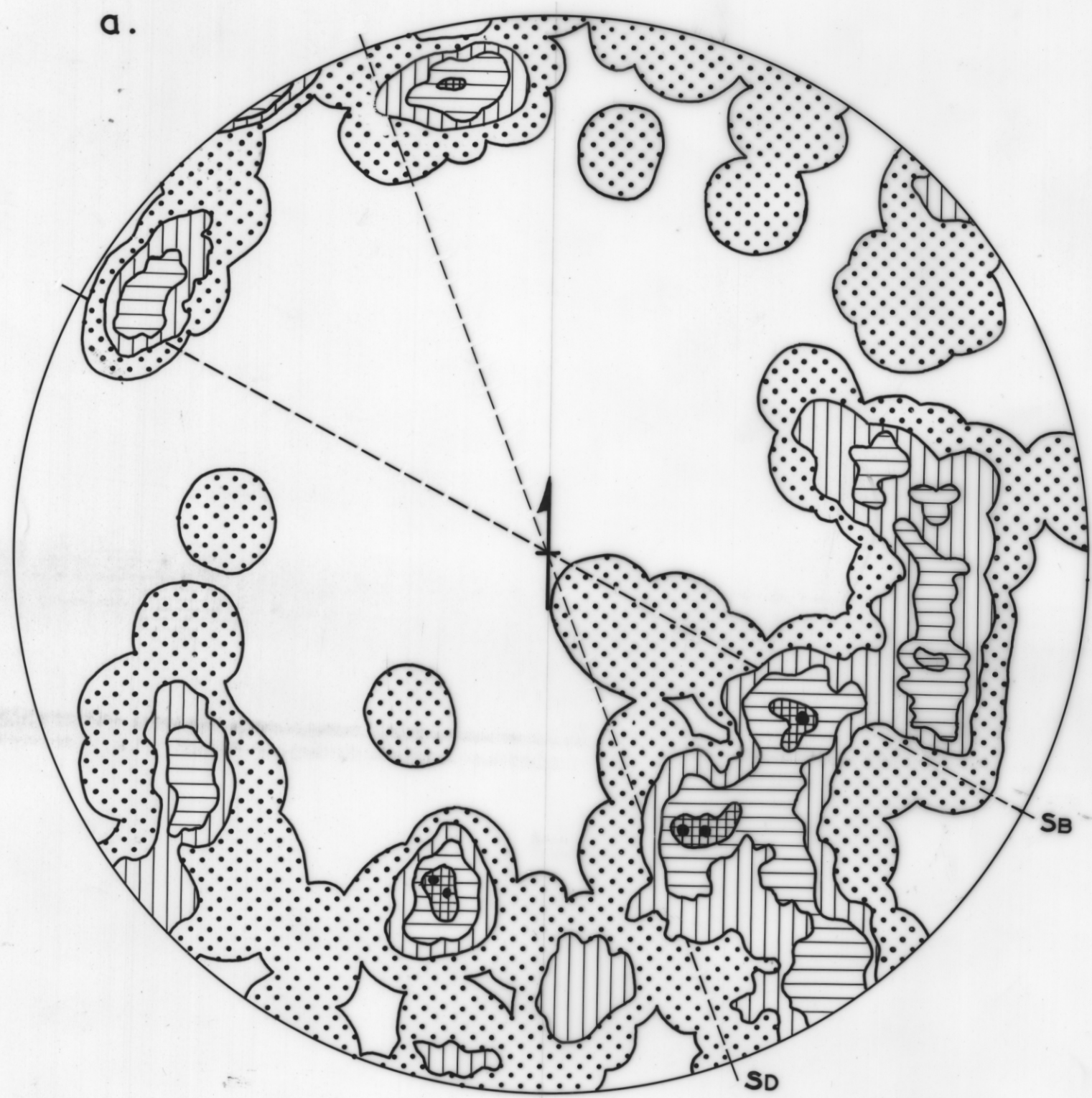
151 QUARTZ (UNDULOSE)
