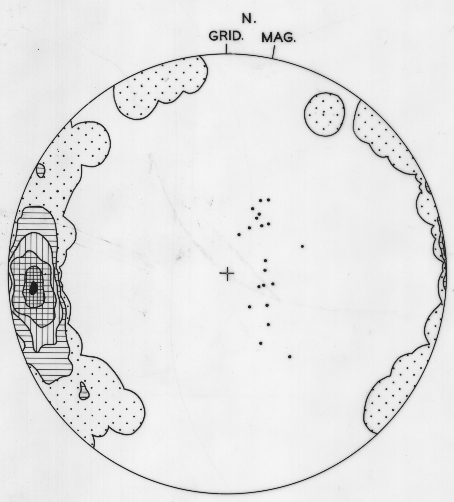
WEST BASIN SxS: P=20 N=190 CONTOURS 0-4-7-8-20-45-50% MAX. 55%
