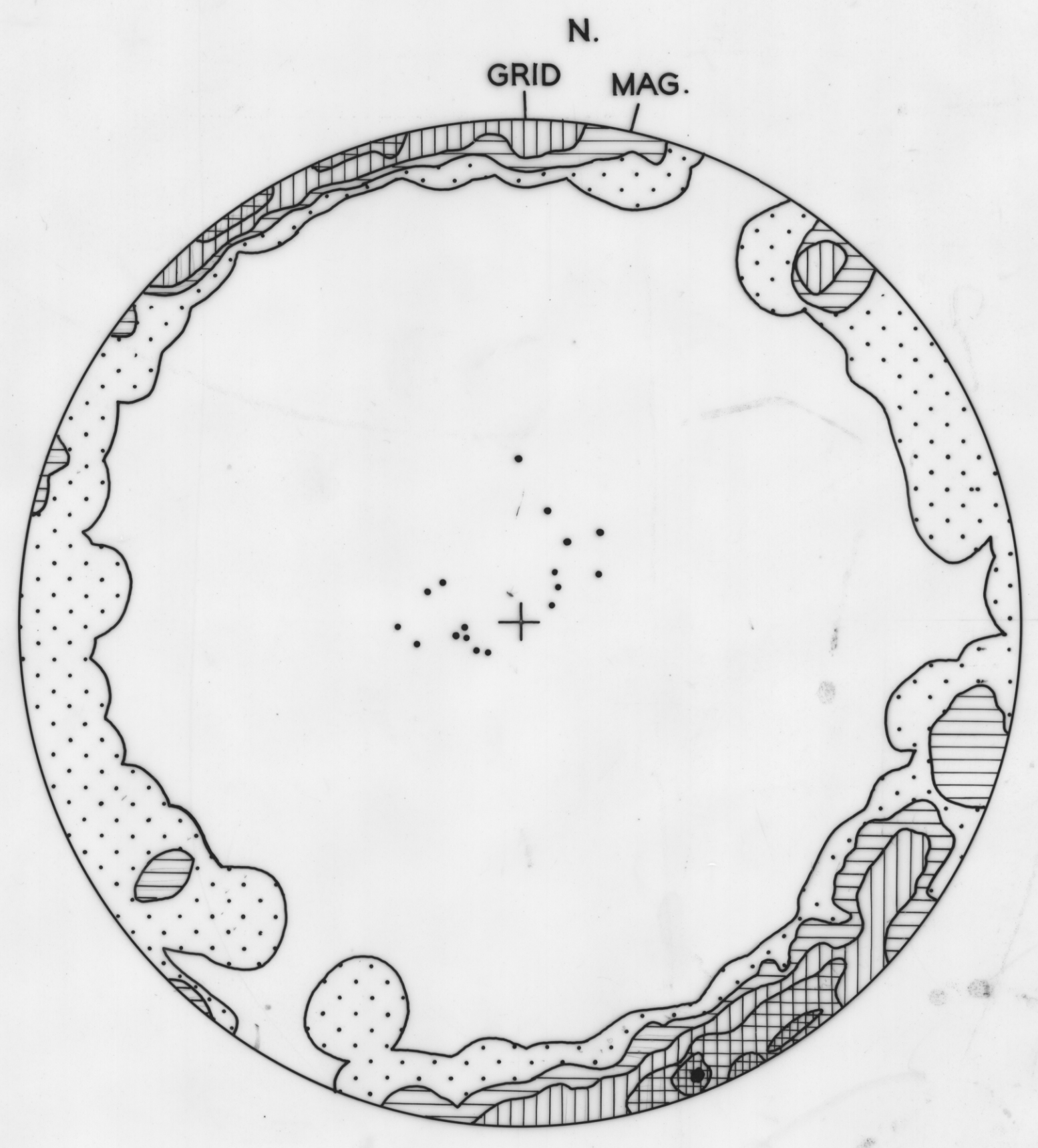
MIDDLE BASIN SxS: P=17 N=136 CONTOURS 0-3-5-5-10-15% MAX. 17%
