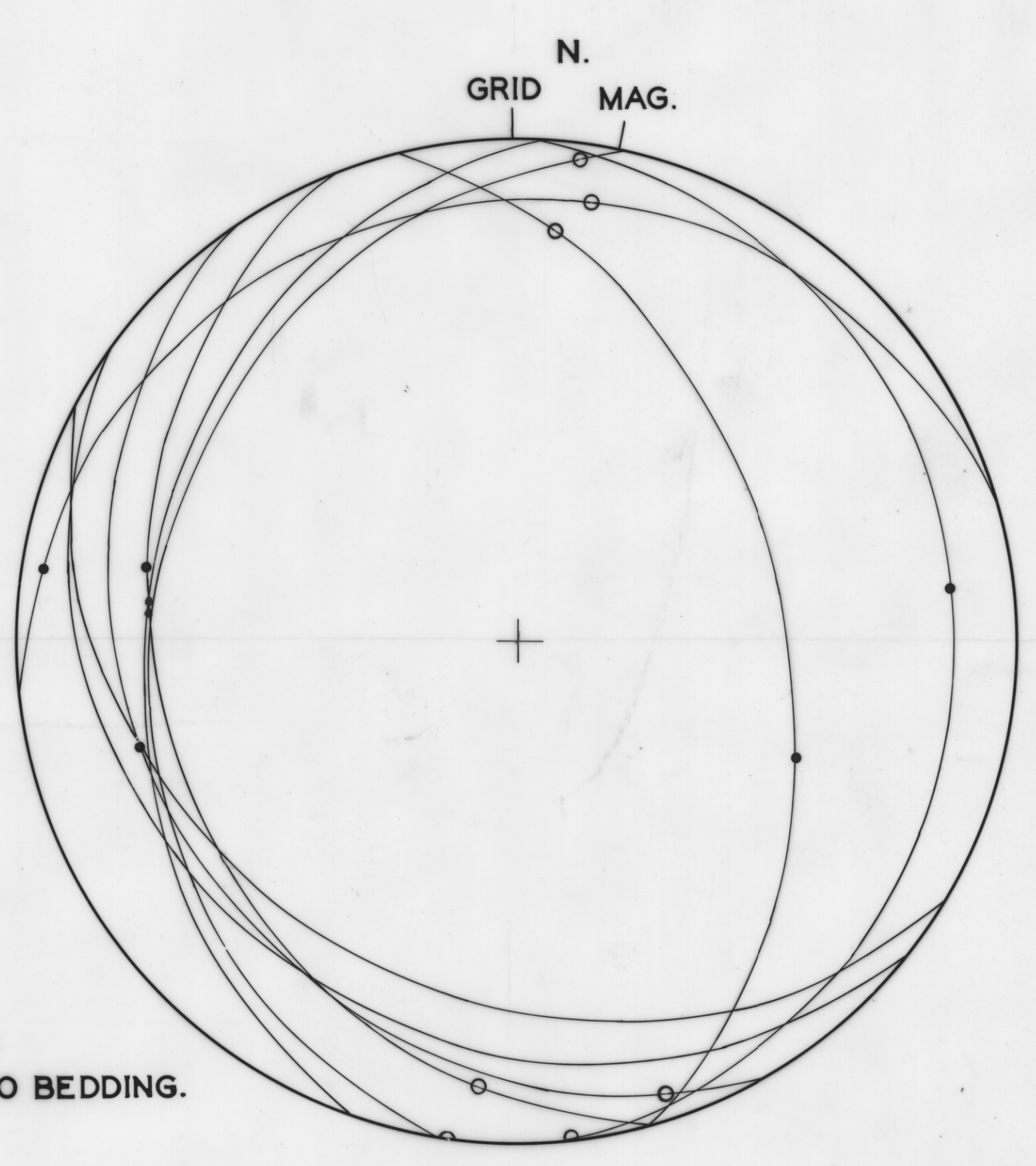
FAULTS ◦ NORMAL TO SLIP IN FAULT ZONE • SLIP
