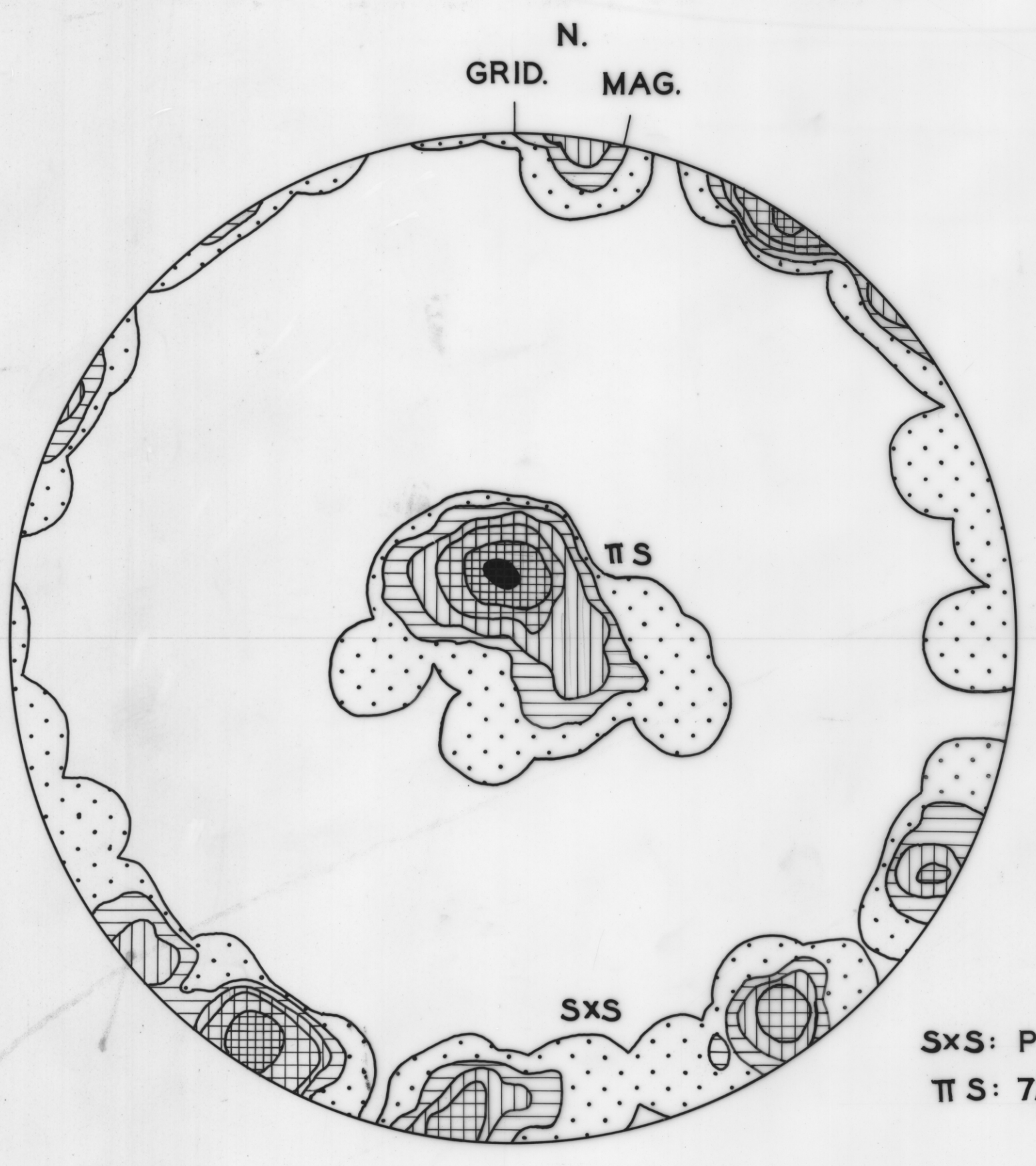
EAST BASIN SxS: CONTOURS 0-5-8-10-20% MAX. 20% TTS: CONTOURS 0-5-10-20-40% MAX. 60%
