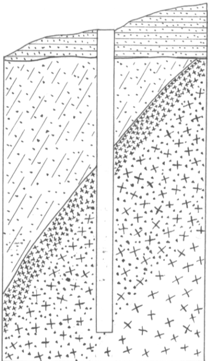
SECTION EXPOSED BY SHAFT AT ROYS-HILL MINE
