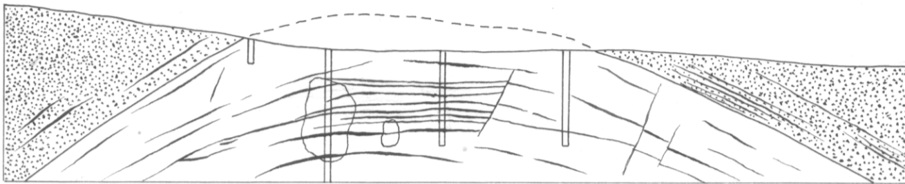
IDEAL SECTION THROUGH GRANITE BOSS OF ZINNWALD SHOWING FISSURES OF CONTRACTION
