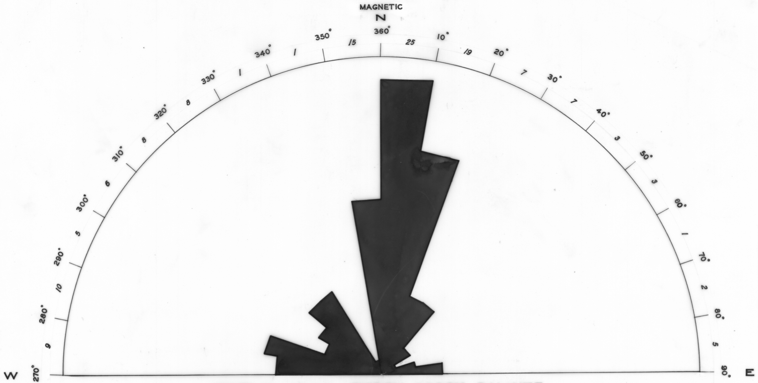
JOINT DIAGRAM — RISDON BROOK DAMSITE NUMBER OF JOINTS SHOWN FOR EVERY 10 DEGREES
