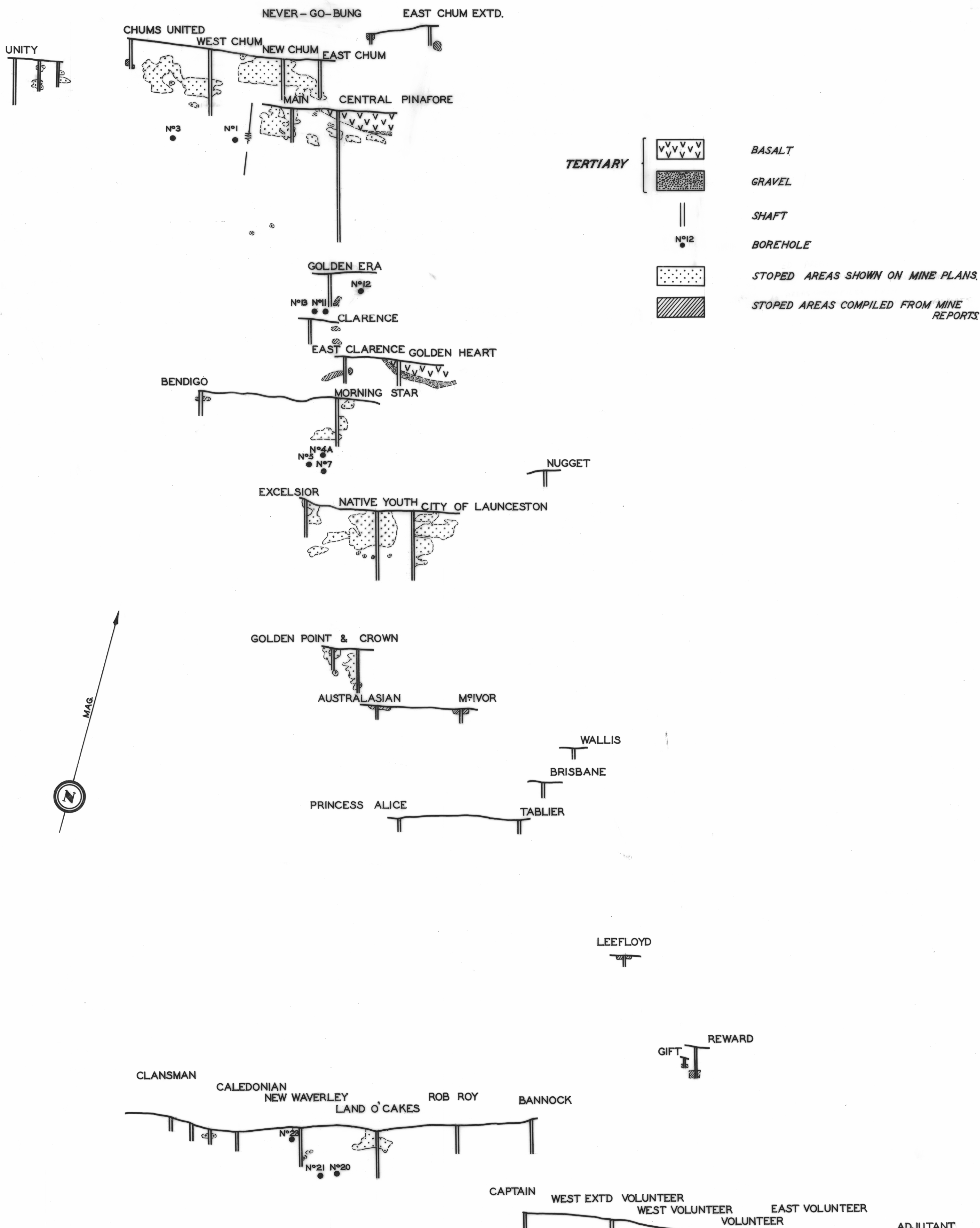
SURFACE BOREHOLES 1935-1938 ASSAYS AT INTERSECTIONS SHOWN ON PLAN.
