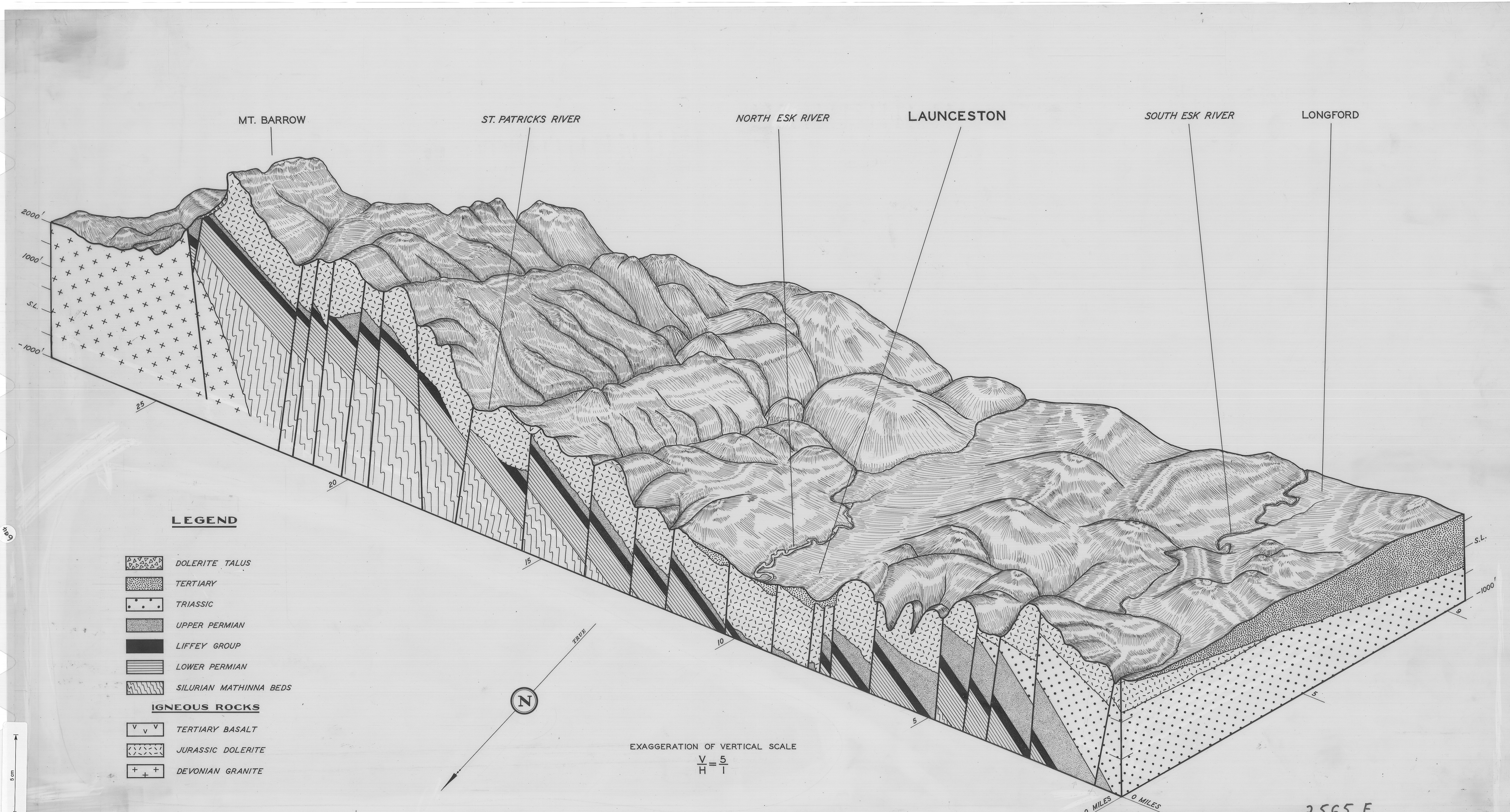
FIG. 12. DEVELOPMENT OF THE TAMAR TROUGH (LAUNCESTON EXPLAN. NOTES) 1966 by M.J. LONGMAN
