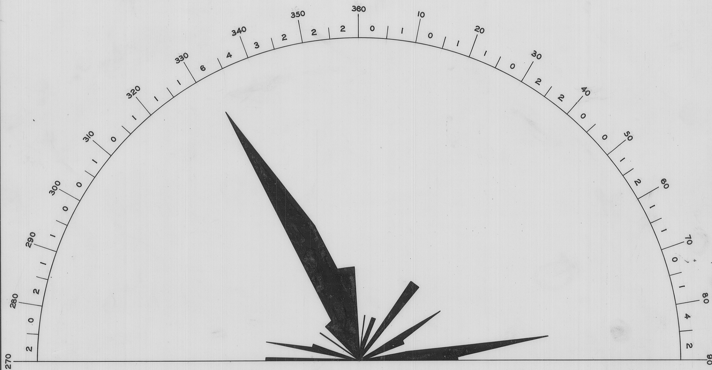
QUARTZ VEINS
