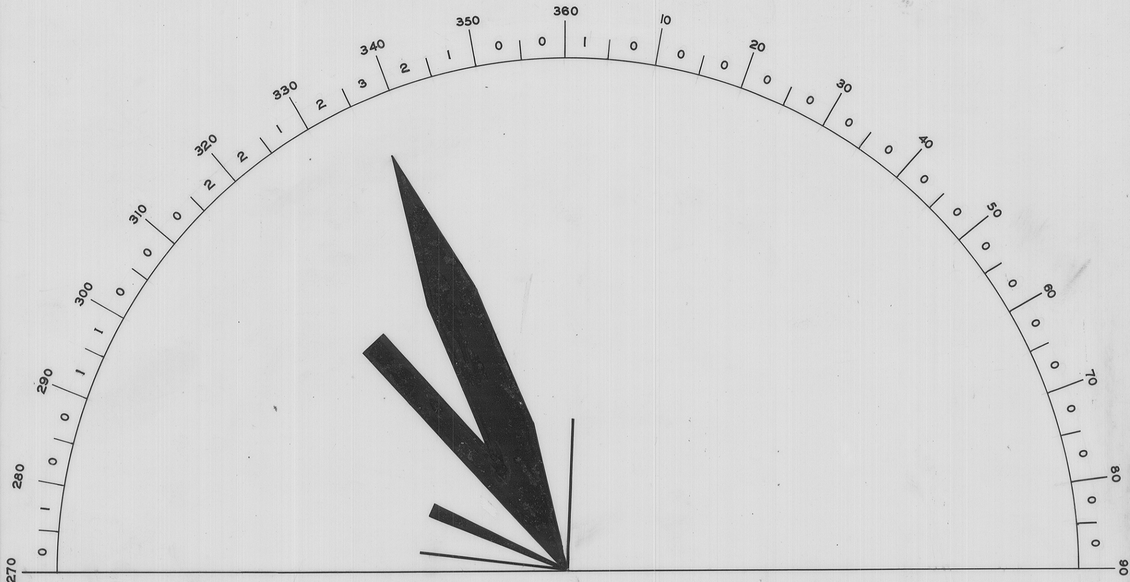
QUARTZ VEINS
