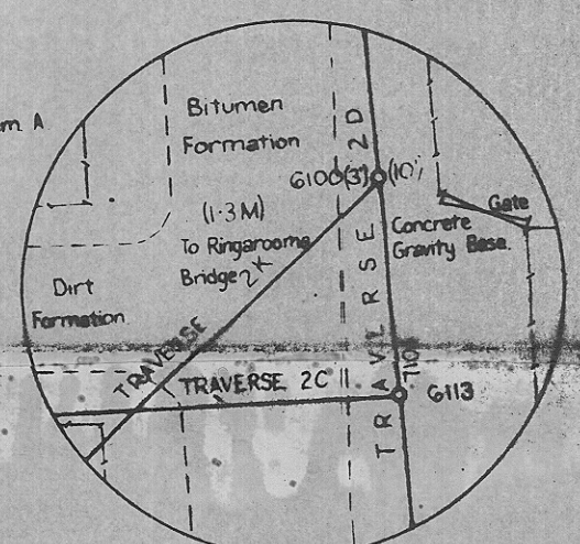
GRAVITY BASE FOR DERBY-WINNALEAH AREA Diagram A (Not to Scale)
