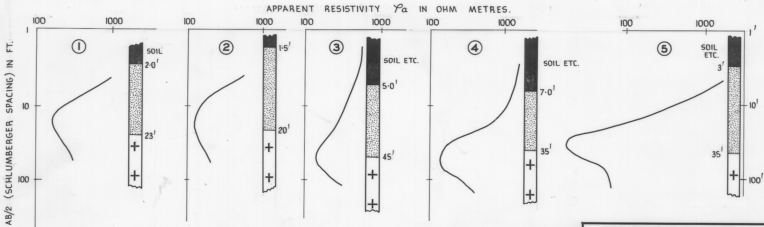
RESISTIVITY PROBES SHOWING INTERPRETATIONS
