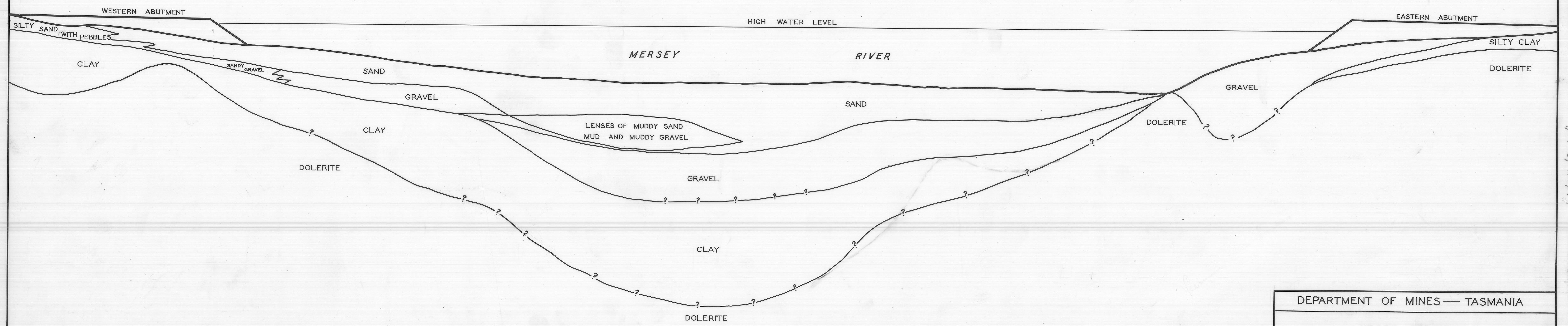
GENERALIZED CROSS SECTION
