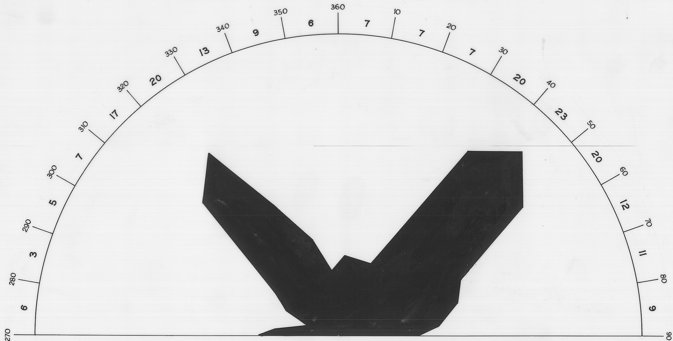
a. INTERNAL PLANAR STRUCTURES IN PORPHYRITIC ADAMELLITE TOTAL 202 READINGS
