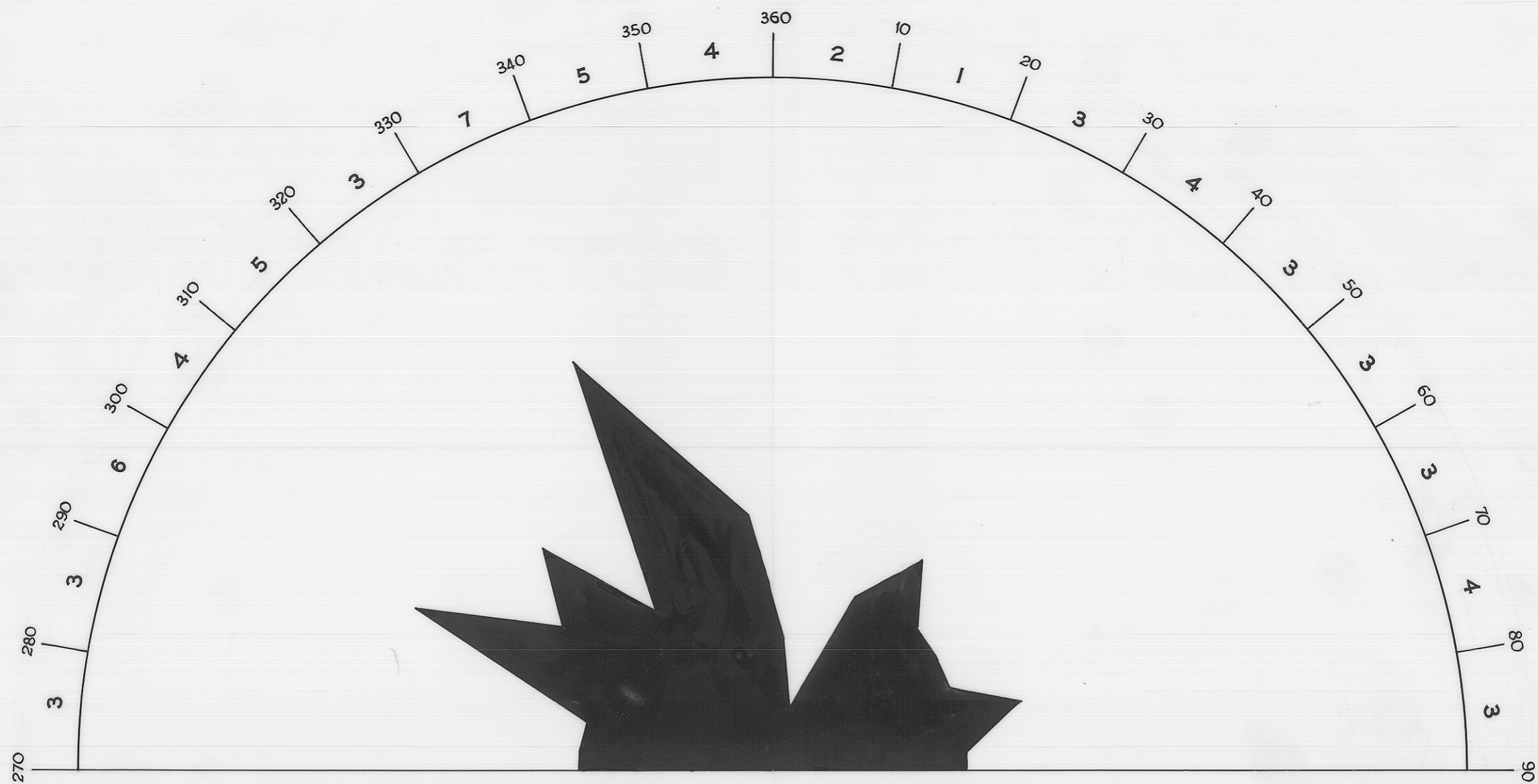
b. STRONGLY DEVELOPED JOINTS IN PORPHYRITIC ADAMELLITE TOTAL 66 READINGS
