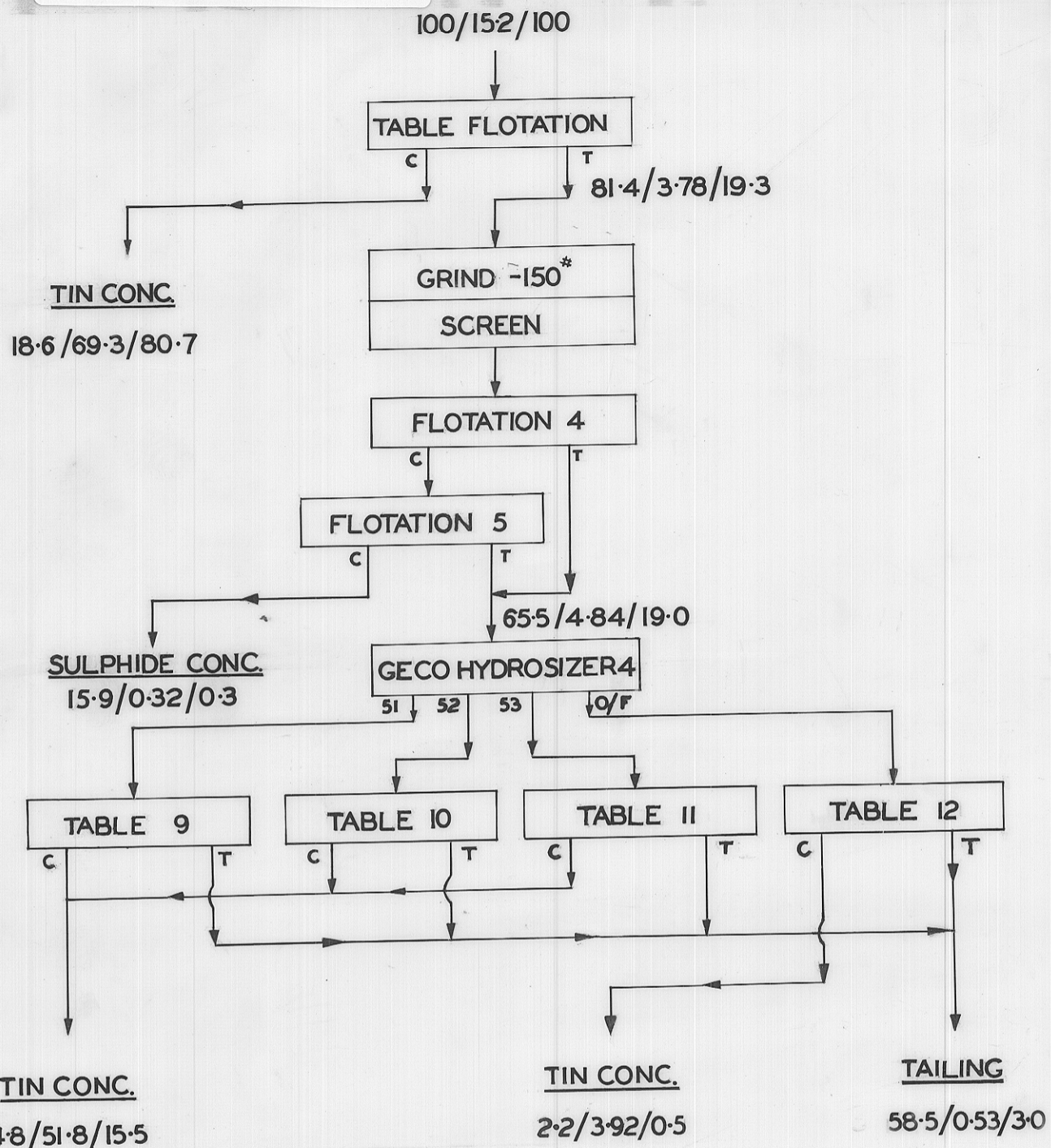
FLWSHEET FOR ROUGHER SAND TABLE CONCENTRATE TREATMENT
