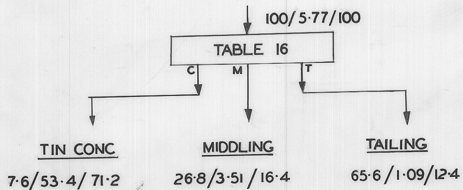
FLWSHEET FOR ROUGHER VANNER CONCENTRATE TREATMENT
