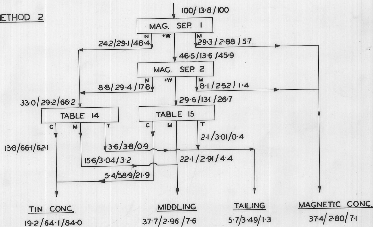
FLWSHEETS SHOWING METHODS OF TREATMENT USED ON SLIME TABLE ROUGHER CONCENTRATE
