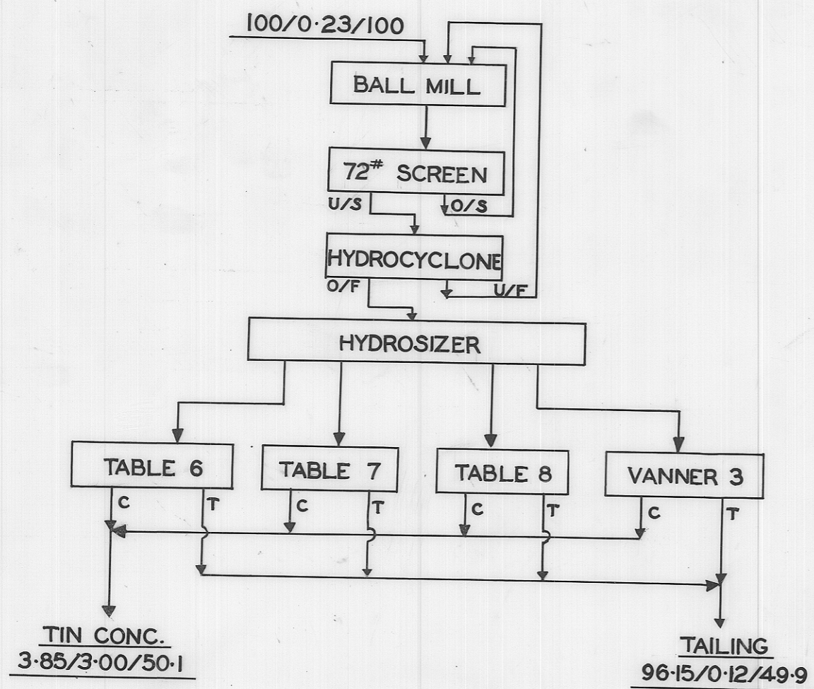
FLWSHEET — N° 1 TABLE MIDDLEING RETREATMENT
