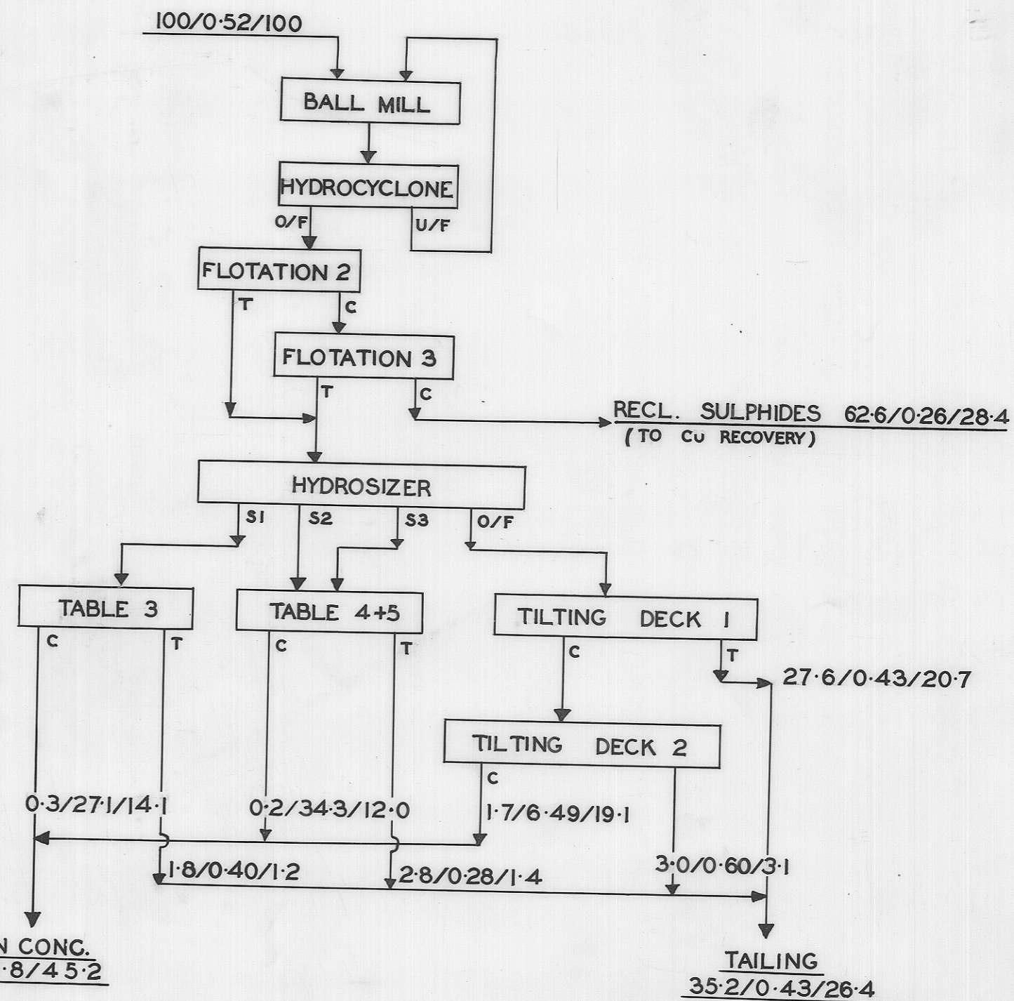
FLWSHEET — ROUGHER SULPHIDE RETREATMENT
