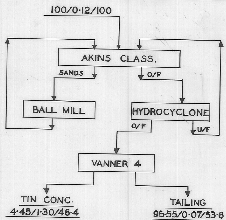
FLWSHEET — N° 2 TABLE MIDDLEING RETREATMENT
