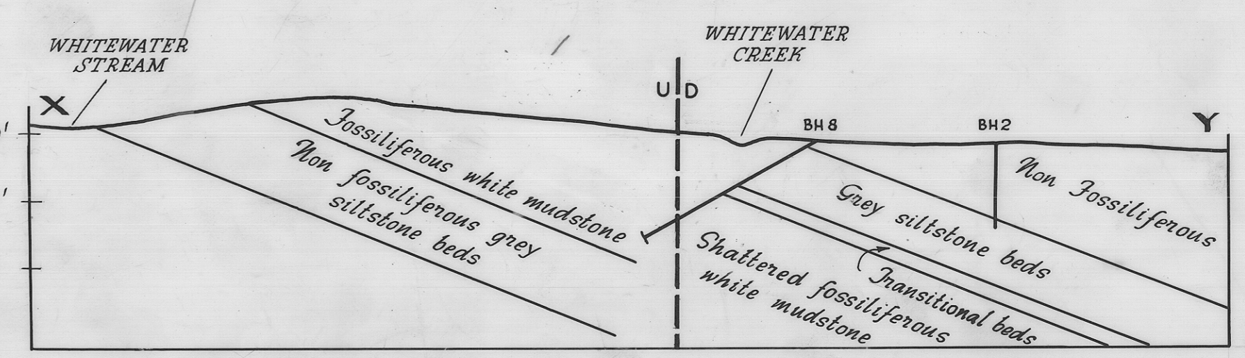
SECTION X-Y
