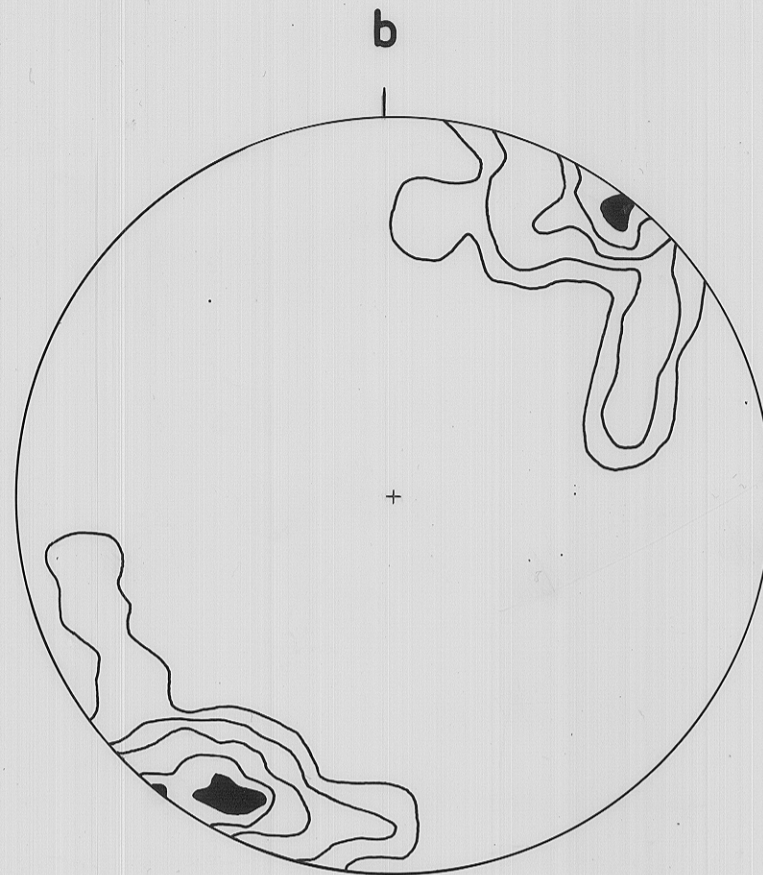
52 poles of P3 fold axes contours 1-6-9-12-15%
