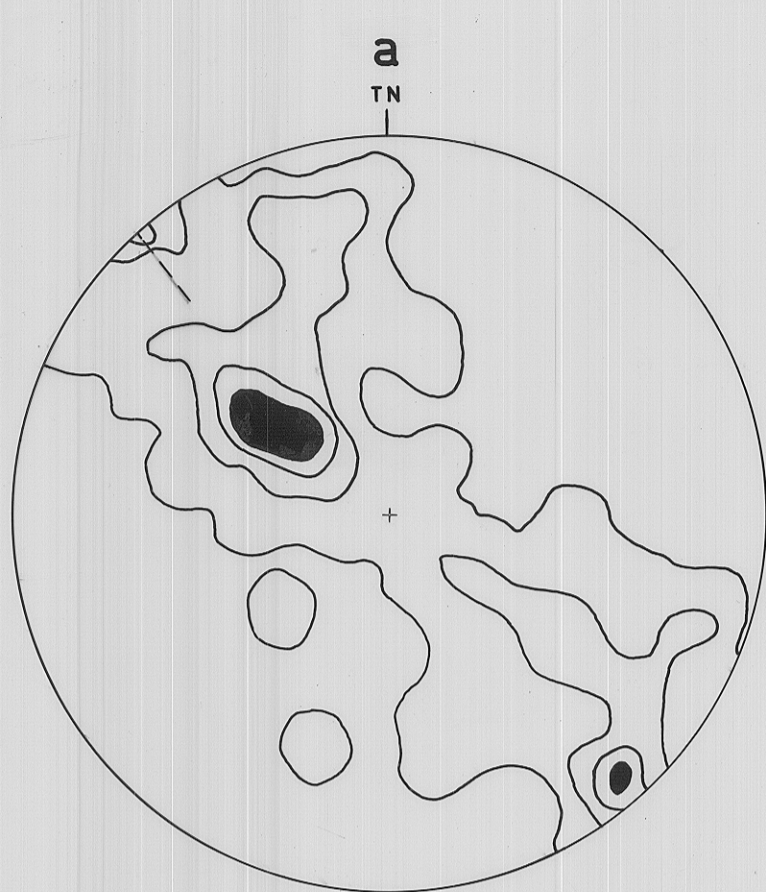
121 poles to bedding contours 1-3-6-9%
