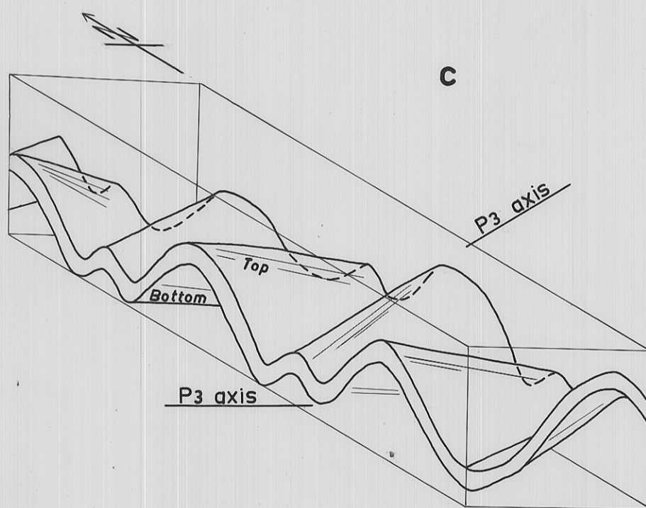
Diagrammatic representation of P3 folds.
