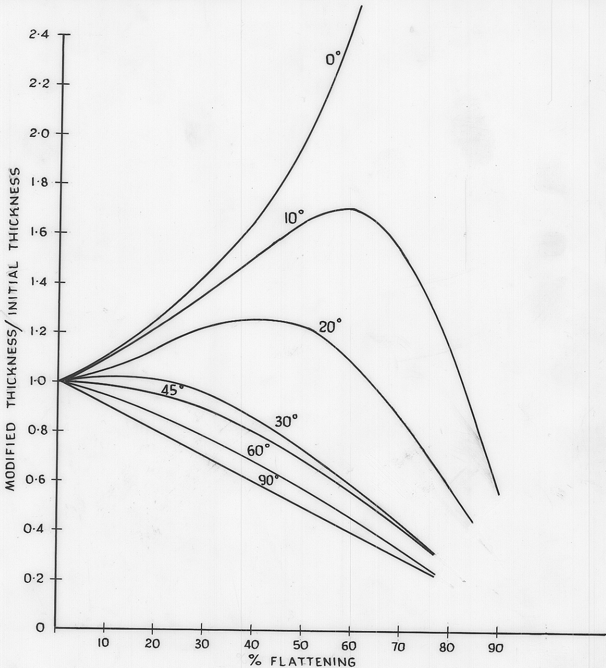
Change in thickness of a layer undergoing passive internal rotation (relative to initial thickness) with uniform flattening, for selected values of initial tilt.
