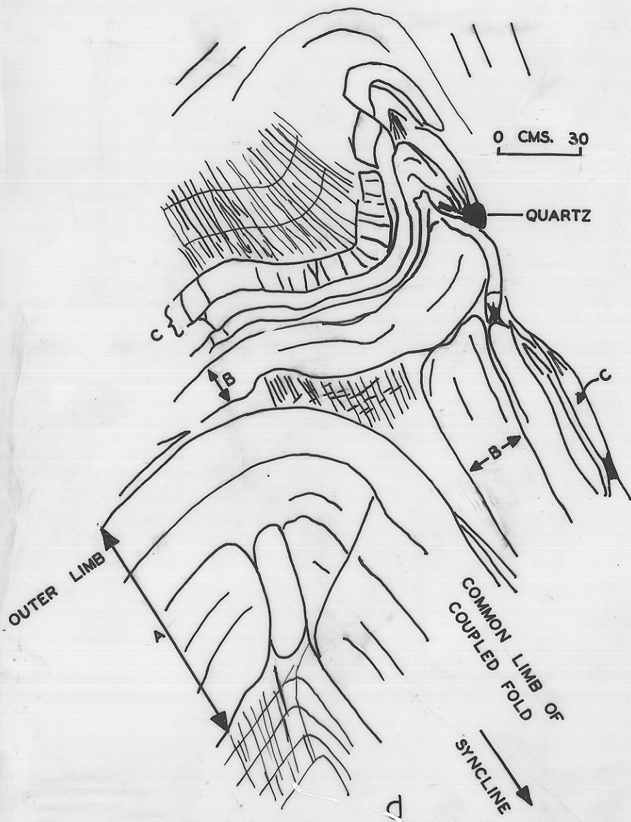
DISHARMONIC FOLD PROFILES FROM SULPHUR CREEK
