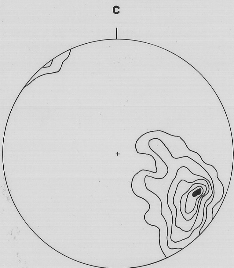
65 poles to P1 axial planes 1-3-6-9-12-15-18%
