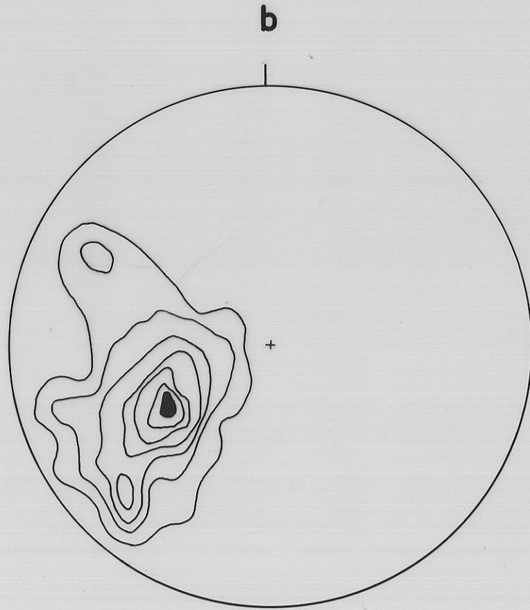
75 poles of P1 fold axes 1-3-6-9-15-21-27%
