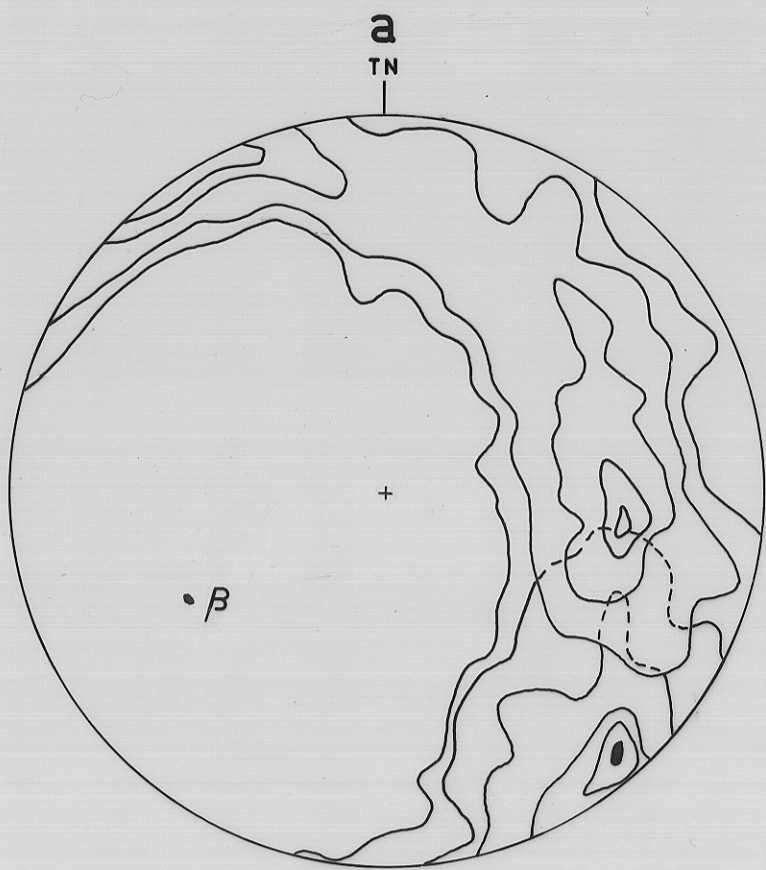
200 poles to bedding contours 1-3-6-9-12-15%
