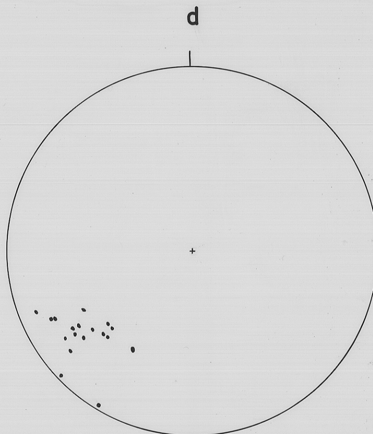
18 poles of P5 fold axes.
