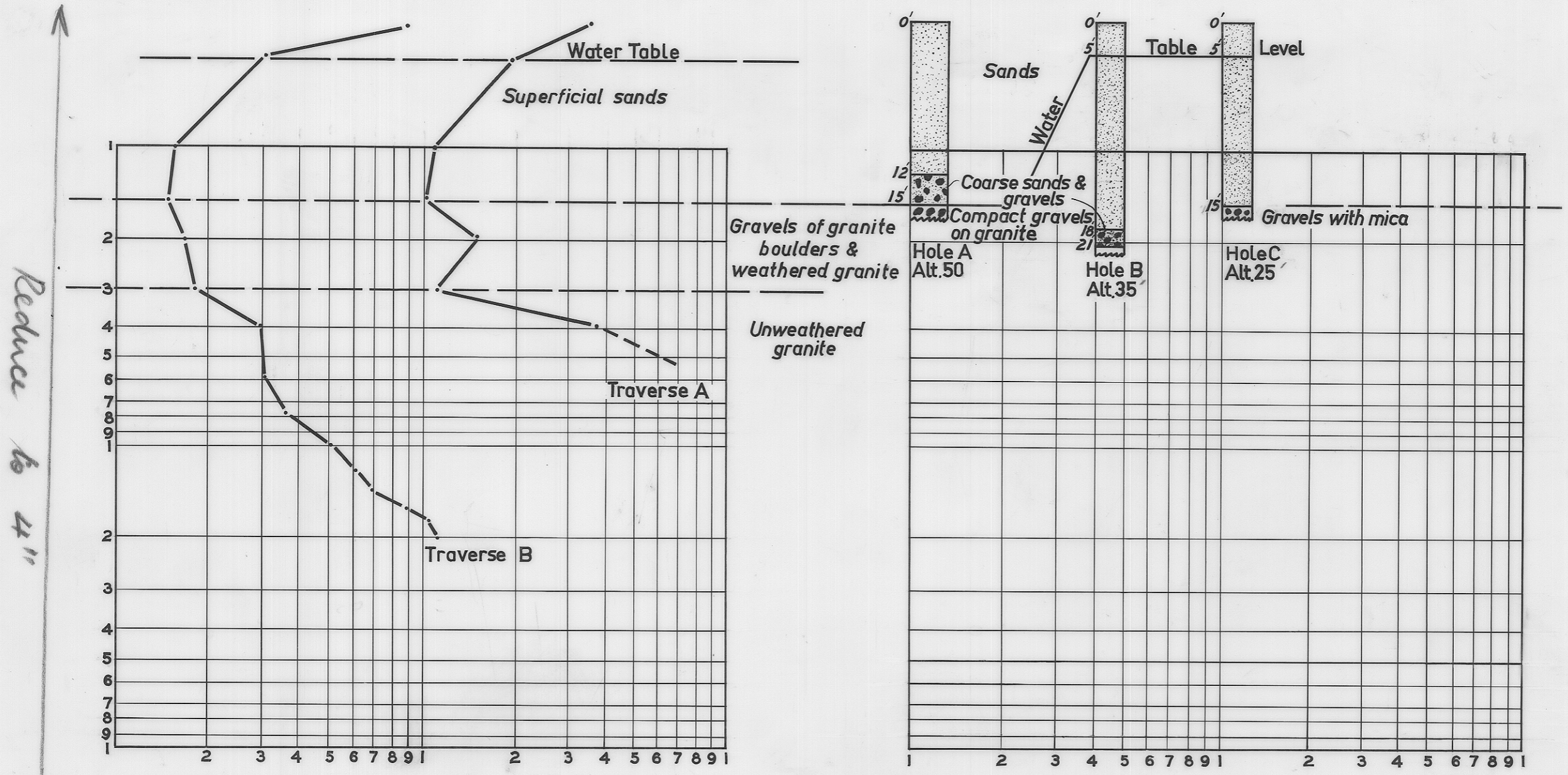
FIG 2 RESISTIVITY PROFILE & DRILL CORES — TOMAHAWK VILLAGE
